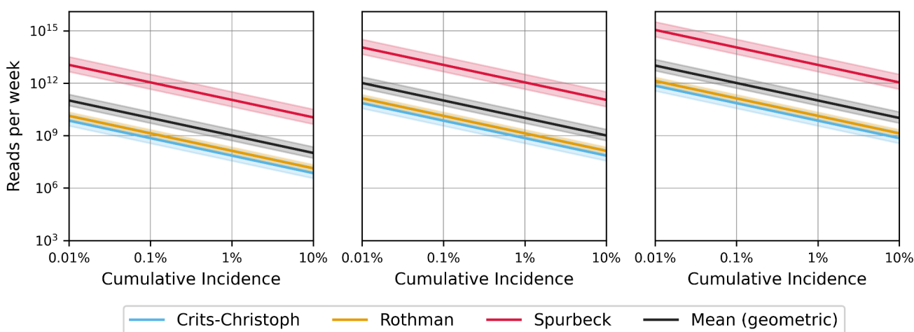
Figure 5: Weekly reads required for detection, given the performance of different study protocols (Crite-Christoph, Rothman, and Spurbeck), and their mean performance. (a) Norovirus (GII), (b) SARS-CoV-2
