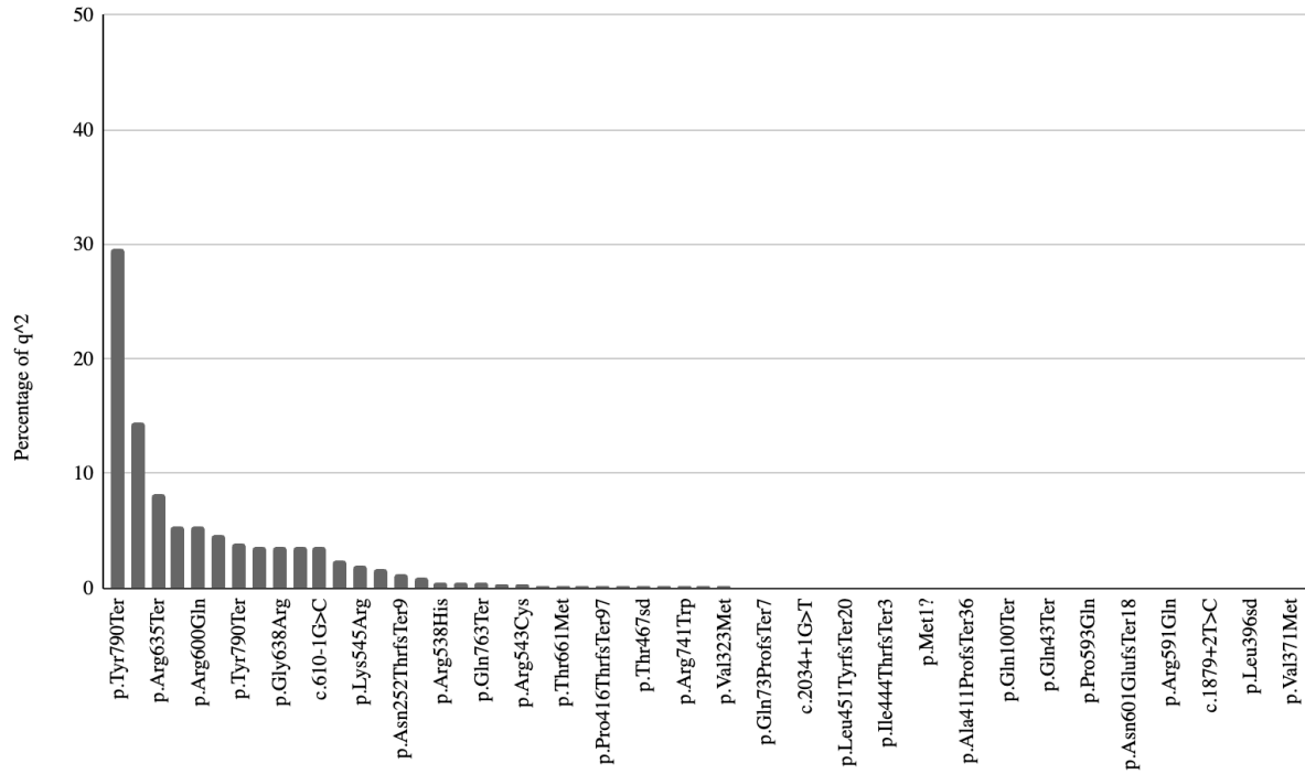
Figure 2D: Percentage of genetic prevalence ( q^2 ) of pathogenic variants in PLA2G6 with non-zero allele frequencies
