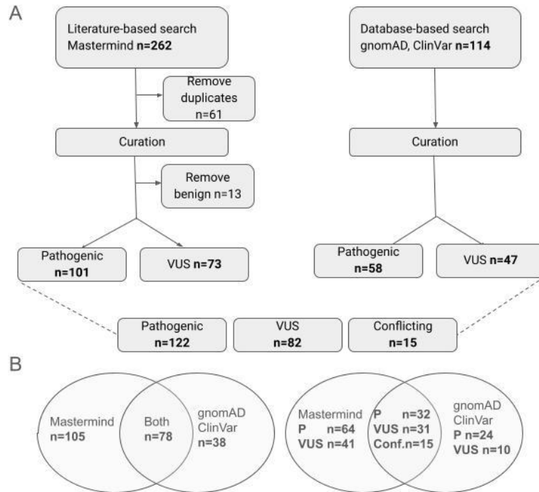
Figure 1. (A) To estimate genetic prevalence of PLA2G6-associated neurodegeneration, we have utilized a literature-based approach (left) and database-based approach (right). In total, 122 pathogenic, 82 VUS, and 15 conflicting variants were curated and classified. (B) Pathogenic and VUS variants recorded by two independent approaches.
