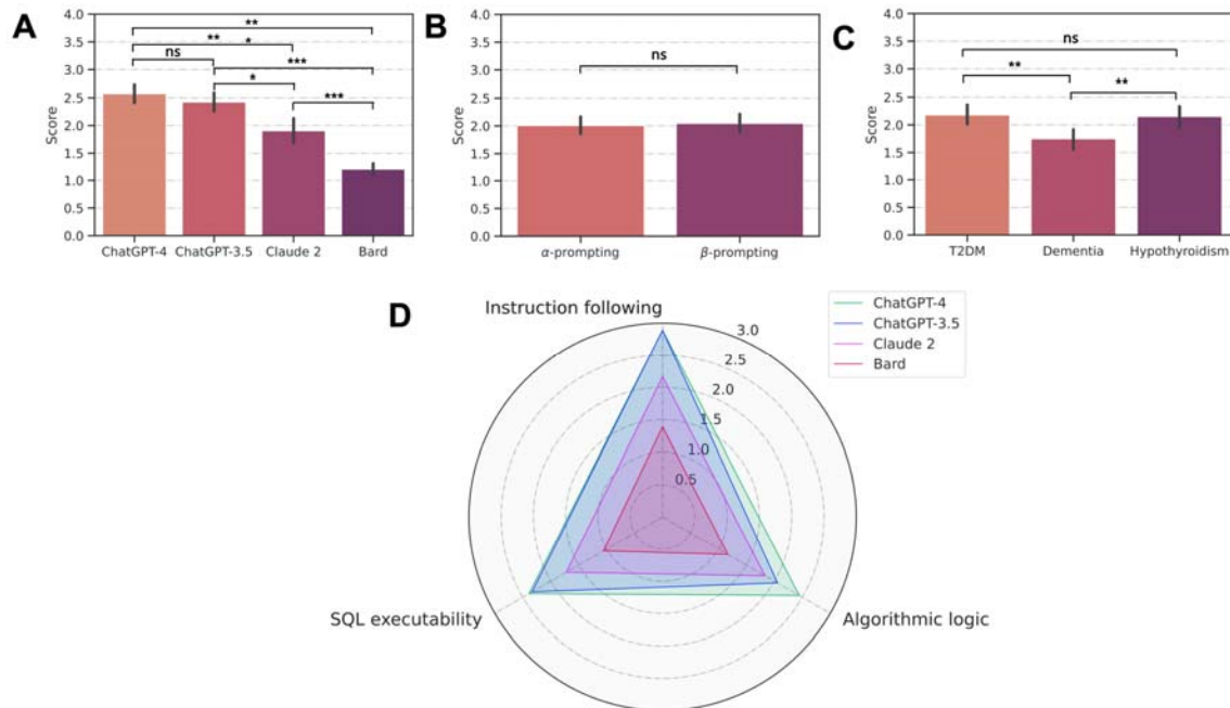
Figure 2. A comparative analysis based on expert evaluations focusing on A) four large language models, B) two prompting strategies, C) three phenotypes, and D) three individual evaluation axes. Numeric scores of 3, 2, and 1 correspond to expert assessments of “Good”, “Medium”, and “Poor”, respectively. ***, **, and * denote p < 0.001 , p < 0.01 , and p < 0.05 , respectively. ns=not significant.
