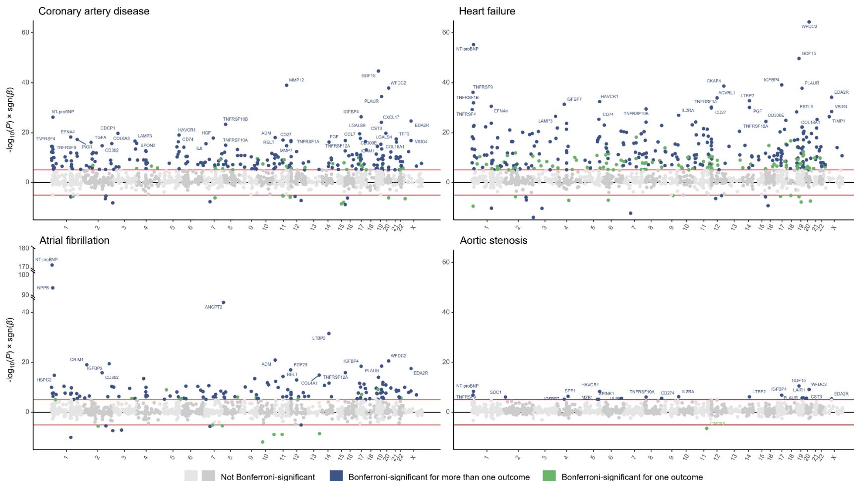
648 Fig. 2. Associations of circulating protein levels with incident coronary artery disease, heart failure, atrial fibrillation, and 649 aortic stenosis.
