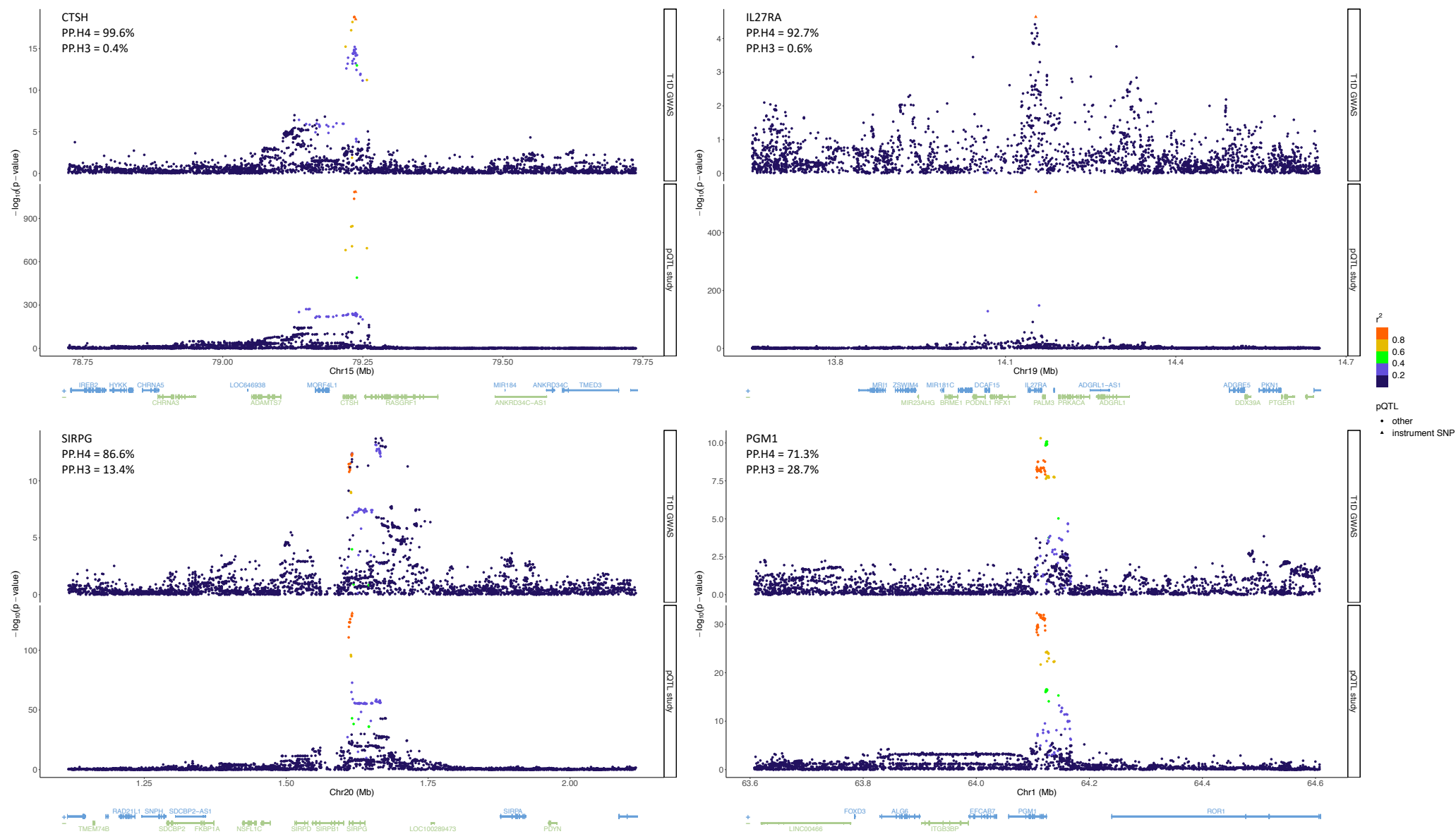
Figure 3. Colocalization of genetic associations with circulating abundances of prioritized target proteins and the risk of type 1 diabetes. The lead cis-genetic instruments are indicated. Genetic variants located in a \pm 500 kb window centered around each genetic instrument are plotted with their significance in respective studies, and colored by the magnitude of correlation (linkage disequilibrium, LD r^2 ) with the corresponding instrument. For each target protein, the posterior probability of colocalization (PP.H4) and the posterior probability of co-existence of two distinct causal variants (PP.H3) are indicated. The UCSC known gene tracks are presented, with gene models colored by their respective strands.
