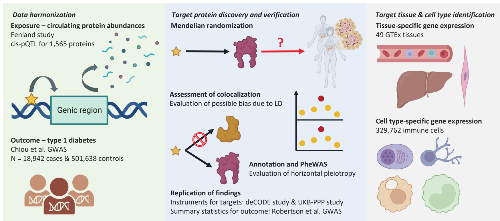
Figure 1. Overview of study. Mendelian randomization (MR) was conducted leveraging genome-wide association studies (GWASs) of circulating protein abundances in the Fenland study as well as a meta-analysis of type 1 diabetes GWASs. Colocalization analyses and evaluation of horizontal pleiotropy through annotation and phenome-wide association study (PheWAS) were conducted to verify MR assumptions. Significant associations were replicated using other proteomic studies and another meta-analysis of type 1 diabetes GWASs. Gene expression enrichment analyses were conducted to identify potential candidate tissues and cell types.
