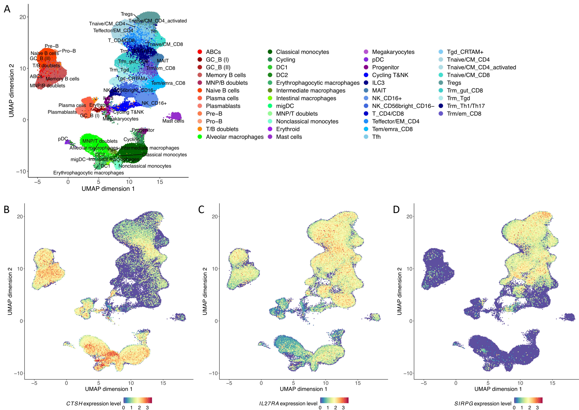
Figure 5. Single-cell gene expression profiles of CTSH , IL27RA , and SIRPG in immune cells. (A) Visualization of 329,762 immune cells based on Uniform Manifold Approximation and Projection (UMAP) of their transcriptomes. Cells are colored by manually curated cell types. Red colors: B cell compartment; Green colors: myeloid compartment; Purple colors: miscellaneous cell types; Blue colors: T cell compartment. Descriptions of cell types are available in Supplementary Table S11. Normalized gene expression levels of (B) CTSH , (C) IL27RA , and (D) SIRPG are visualized. UMAP coordinates, cell type annotations, and normalized gene expression levels were obtained from the Single Cell Portal ( https://singlecell.broadinstitute.org/single_cell ) under the accession ID SCP1845.
