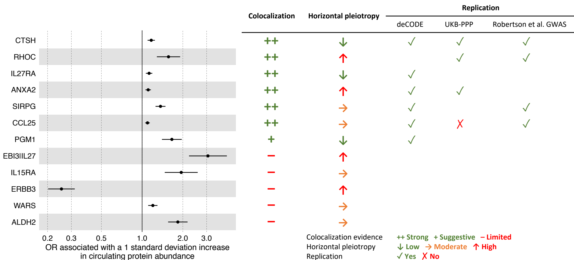
Figure 2. Target protein prioritization. Associations between circulating protein abundances and type 1 diabetes risk that withstood Bonferroni correction of multiple testing are illustrated. Target proteins are ordered by posterior probability of colocalization (Supplementary Table S4). A posterior probability of colocalization > 80% was considered strong evidence of colocalization, while a posterior probability of colocalization > 50% was considered suggestive evidence of colocalization. Risk of horizontal pleiotropy was assessed using V2G scores for quantifying functional connections between genetic instruments and target protein-coding genes, as well as phenome-wide associations for exploring potential pleiotropic pathways (Methods). Associations supported by strong or suggestive colocalization evidence were replicated using additional resources (Methods). Blank space indicates that no genetic instrument or proxy was identified to replicate the association. Target proteins were prioritized based on strong or suggestive colocalization evidence, the absence of a high risk of horizontal pleiotropy, and the consistent replication of associations with the risk of type 1 diabetes.
