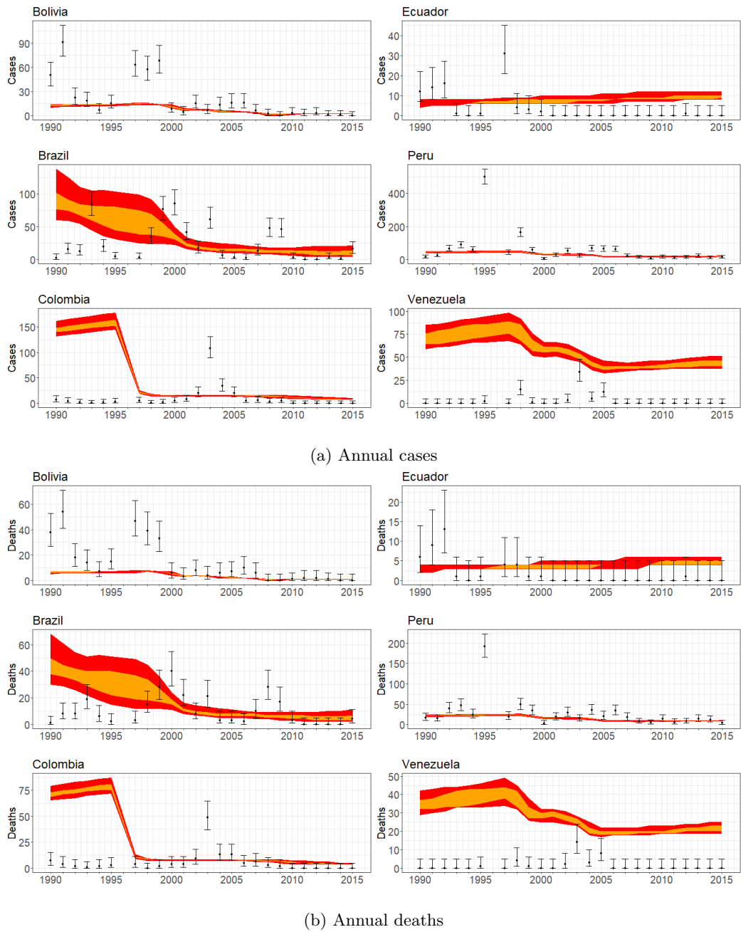
Figure 3: Graphs showing reproduction of selected South American annual case (a) and death (b) data using 1000 parameter sets drawn from post-burn-in distribution obtained from 4 Markov chains. Points show real data (error bars obtained from binomial confidence interval calculations using the population); orange regions show distribution of 50% of results, red regions show distribution of 95% of results.
