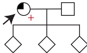
Family 4 (p.Arg1305Cys)
