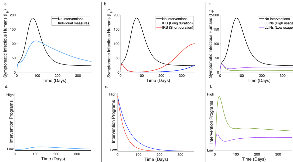
Figure 5: Simulation results capturing the impact of IRS, LLINs, and individual preventive measures on symptomatic infectious humans over a period of 365 days. a. Results comparing the impacts of individual measures on symptomatic malaria cases with the baseline when no interventions are implemented. b. Results comparing the impacts of IRS (long and short duration) with the baseline of no intervention measures on symptomatic infectious cases. c. Results comparing the impacts of LLINs (high and low usage) with no interventions on symptomatic infectious cases. d.–f. Graphical representation of the levels of interventions considered in the simulation studies in a.–c. respectively.
