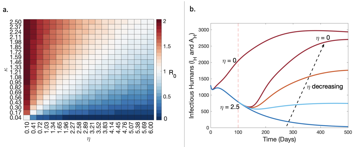
Figure 3: a. A sensitivity analysis of \mathcal{R}_0 on the intervention parameters \kappa and \eta . The colour bar represents \mathcal{R}_0 values ranging from 0 (blue) indicating a negative growth of the disease to 2 (red) indicating a positive initial disease growth. The subplot a. is derived from the solution to Equation (2). b. Simulation results comparing the dynamics of infectious human cases from a steady declining situation (dark blue line), as the recruitment rate of intervention programs is decreased at 100 days compared to having \eta = 0 from the start. Four decreasing scenarios of \eta are considered at 100 days from \eta = 2.5 (dark blue line) to \eta = 0 (dark red line) with \kappa = 0.17 in all scenarios. Results in subplot b. are obtained by solving Equation (1) and recording changes in Equations (1e) and (1f) as \eta varies.
