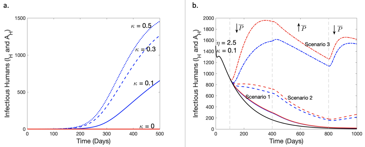
Figure 4: Simulation results exploring how variations in interventions affect infectious trends. a. After-elimination scenarios on how the management (decay) of intervention strategies can affect infectious human cases in the first 500 days post-elimination. After elimination, we set \eta = 0 and consider four scenarios of \kappa ; \kappa = 0 (red solid line), \kappa = 0.1 (blue solid line), \kappa = 0.3 (blue dashed line) and \kappa = 0.5 (blue dotted line). b. The impact of time-varying intervention strategies on malaria-infectious human cases. The solid black line represents the ideal (baseline) scenario with a constant supply and decay rate of interventions, the blue line represents results from variations in the recruitment rate of intervention strategies, \eta , while the red lines represent simulation results from a corresponding change in the decay rate of interventions, \kappa . The changes are chosen such that \bar{P} , (i.e. P at the DFE) for each change in \eta and \kappa is equal. We consider three scenarios of unsteady intervention strategies from day 100 and explore further variations in the supply and decay rate of interventions from days 400 and 800. These days are marked by the vertical grey dashed lines. Scenario 1 is marked by the solid red and blue lines, Scenario 2 by the dashed lines, and Scenario 3 by the dash-dotted lines (specific details are discussed in the main text). Solution of both subplots a. and b. are obtained by solving the model system in Equation (1) and recording the specific changes in Equations (1e) and (1f).
