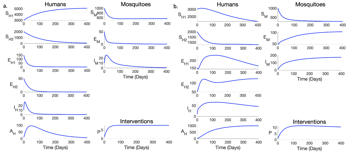
Figure 6: Example model simulation results, showing human and mosquito population dynamics. a. Example simulation result of the model at \mathcal{R}_0 = 0.35 . b. Simulation result of the model at \mathcal{R}_0 = 2.26 . The baseline values given in Table 1 are employed as parameter values for the \mathcal{R}_0 < 1 simulation result, while setting \delta = 3 , \psi_H = 0.5 and \psi_M = 0.5 for the \mathcal{R}_0 > 1 simulation. The initial conditions was set at (S_{H1}(0), S_{H2}(0), E_{H1}(0), E_{H2}(0), I_H(0), A_H(0), S_M(0), E_M(0), I_M(0), P(0)) = (3000, 2000, 150, 50, 10, 10, 1000, 50, 10, 1) .
