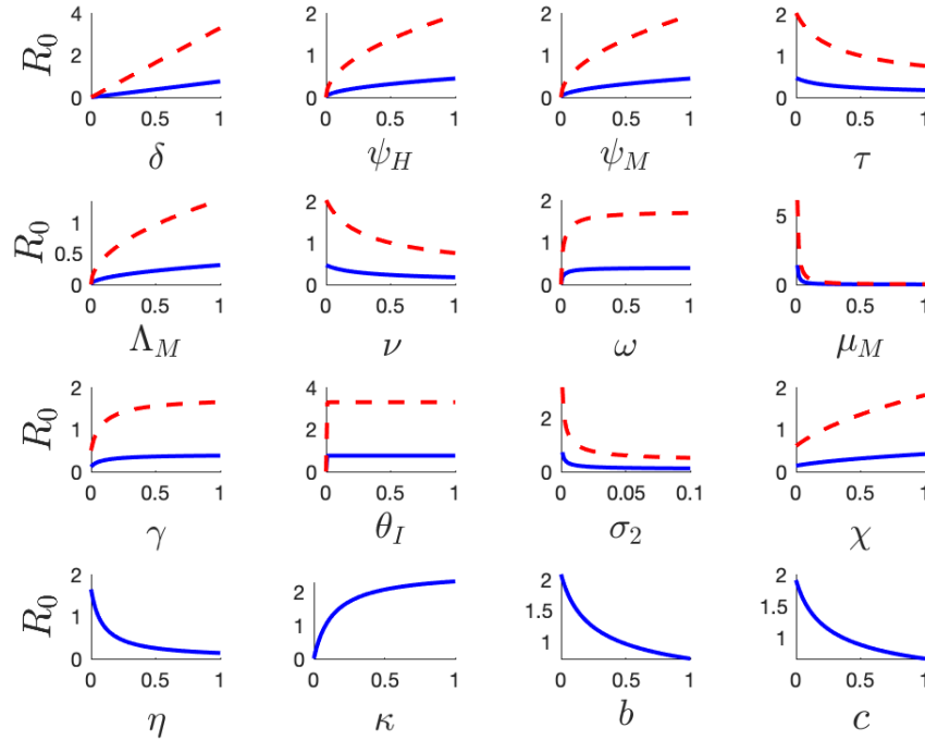
Figure 2: Plots from a local sensitivity (see Equations (2) and (5)) analysis conducted on the model. In these plots, the blue solid lines illustrate the variations in \mathcal{R}_0 , as individual parameters change, whereas the red dashed curves illustrate the variations in \mathcal{R}_0^* with respect to the specific parameter being analyzed, with all other parameters maintained at their baseline values as detailed in Table 1.
