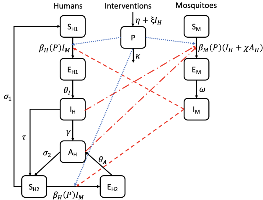
Figure 1: A compartmental diagram of the host-vector model. The red dash-dotted lines represent transmission from infectious humans to susceptible mosquitoes, the red dashed lines represent transmission from infectious mosquitoes to susceptible humans and the blue dotted lines symbolise the effect of intervention strategies on the transmission of malaria in both host and vector populations. Birth and death rates are not presented in this figure, though they are accounted for in the model. Refer to Table 1 for the definitions of the parameters of the model.
