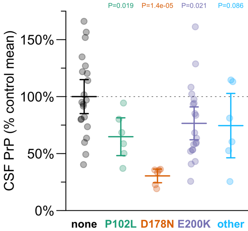
Figure S2. CSF PrP concentration by PRNP mutation.
