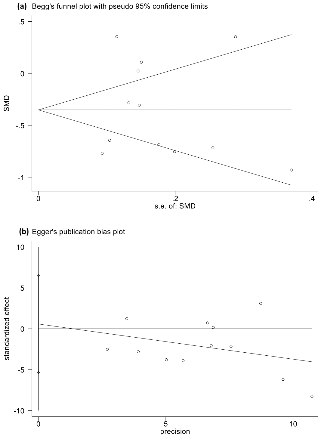
Fig. 6 The funnel plot and Egger's bias plot of publication bias in pooled SMDs analysis of all studies ( a and b ).
