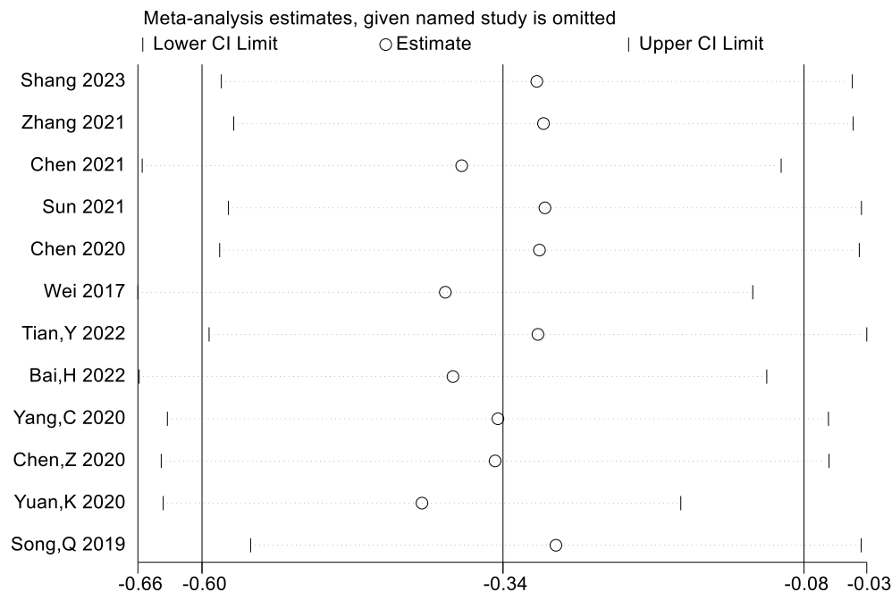
Fig. 3 The provided study was taken away from the forest plot in the current meta-analysis's sensitivity analysis.
