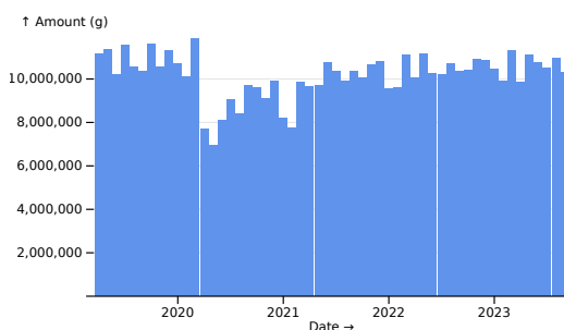
Paracetamol
