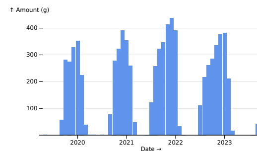
Palivizumab
