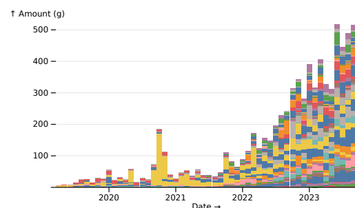
Erenumab
