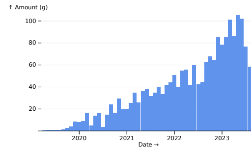
Semaglutide
