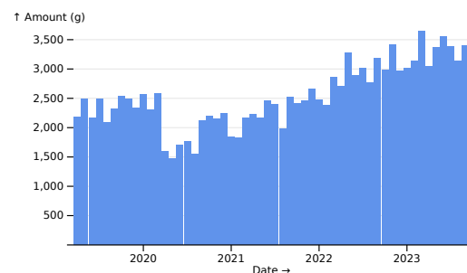
Methylphenidate hydrochloride
