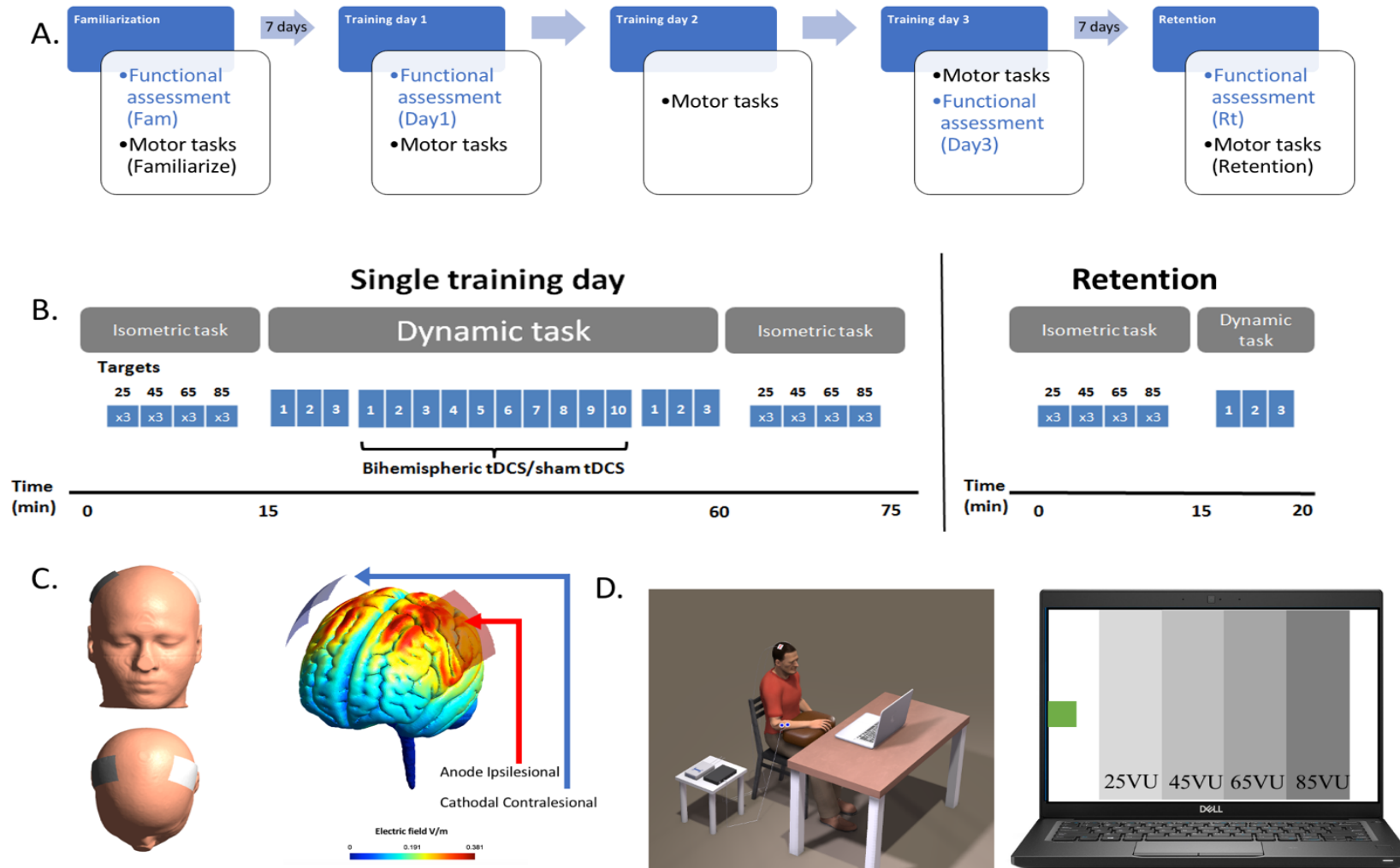
Figure 2. A. Overall study protocol; B. Training protocol for a single training day and the retention test; C. Electrodes placement and electric field modelling; D. Training setup for the MCI tasks and the feedback screen.
