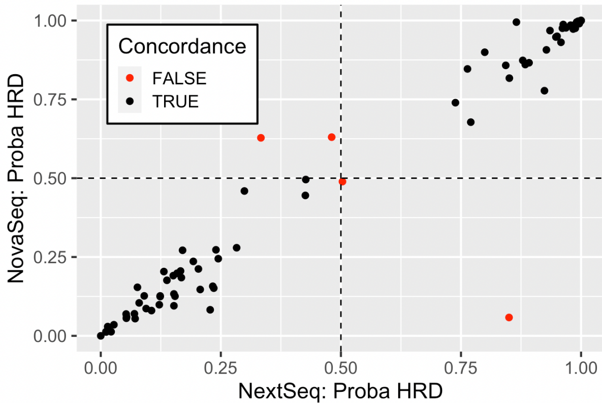
Supplementary Figure 1: Comparison of the HRD probabilities obtained with the NovaSeq 6000 and NextSeq 550 sequencing systems. A total of 90 out of 94 provided consistent HRD status results.
