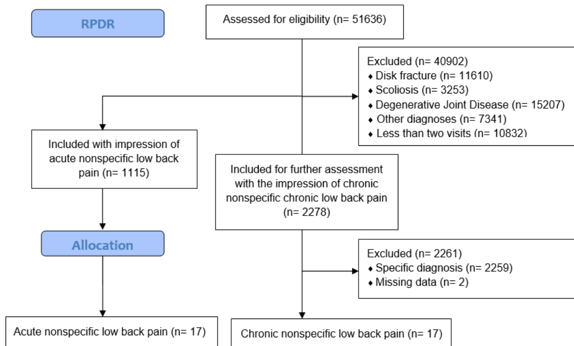
Figure 1. Recruitment Flowchart
