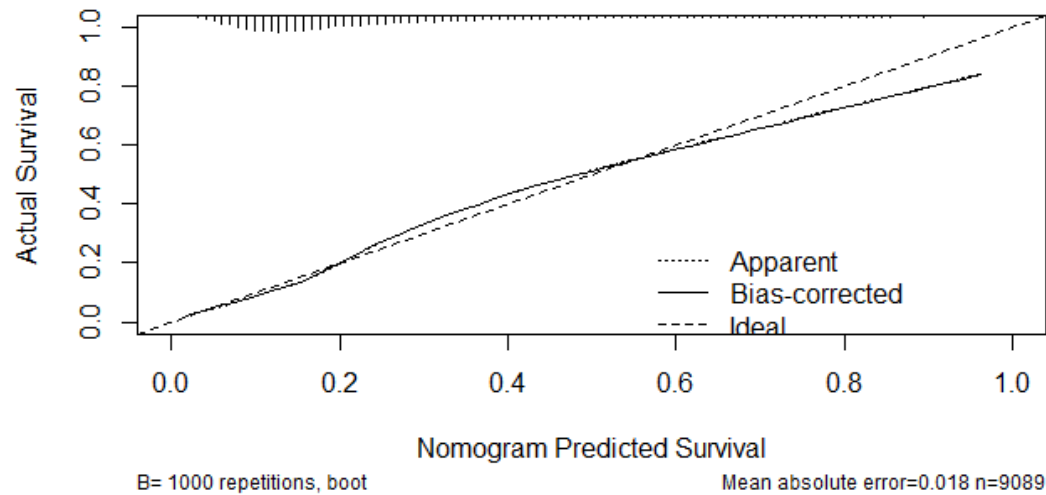
5 Figure 6. The calibration curve of nomogram 1.
