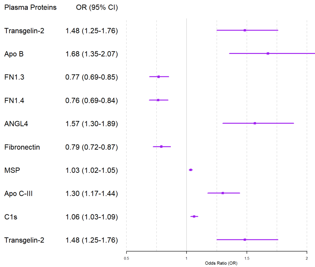
Fig. 2 Results of selected proteins with single snp
