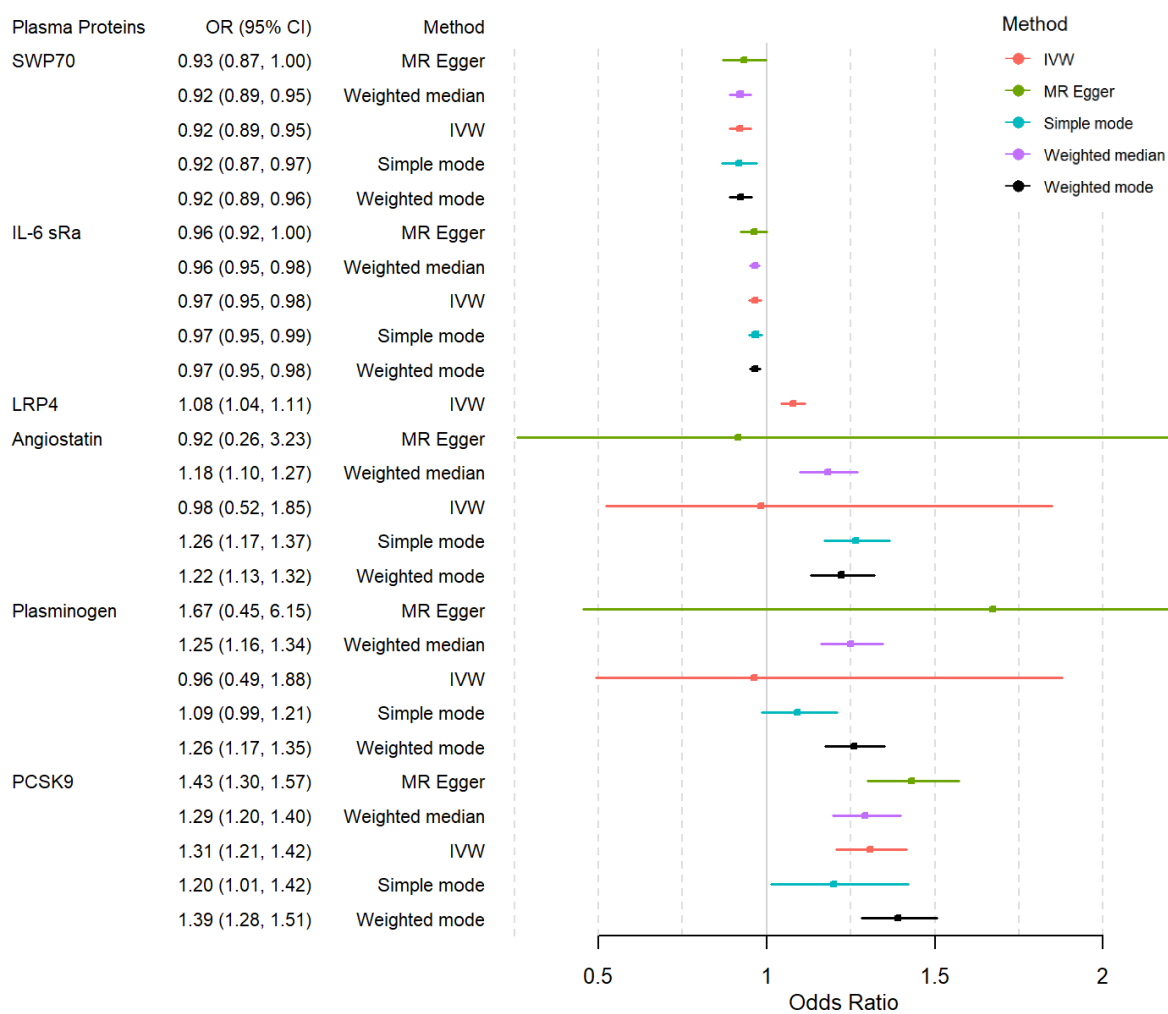
Fig. 3 Results of selected proteins with several snps
