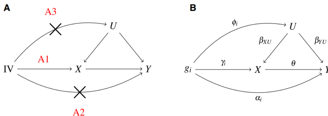
1 2 Fig. 1 The working principle of Mendelian randomization
