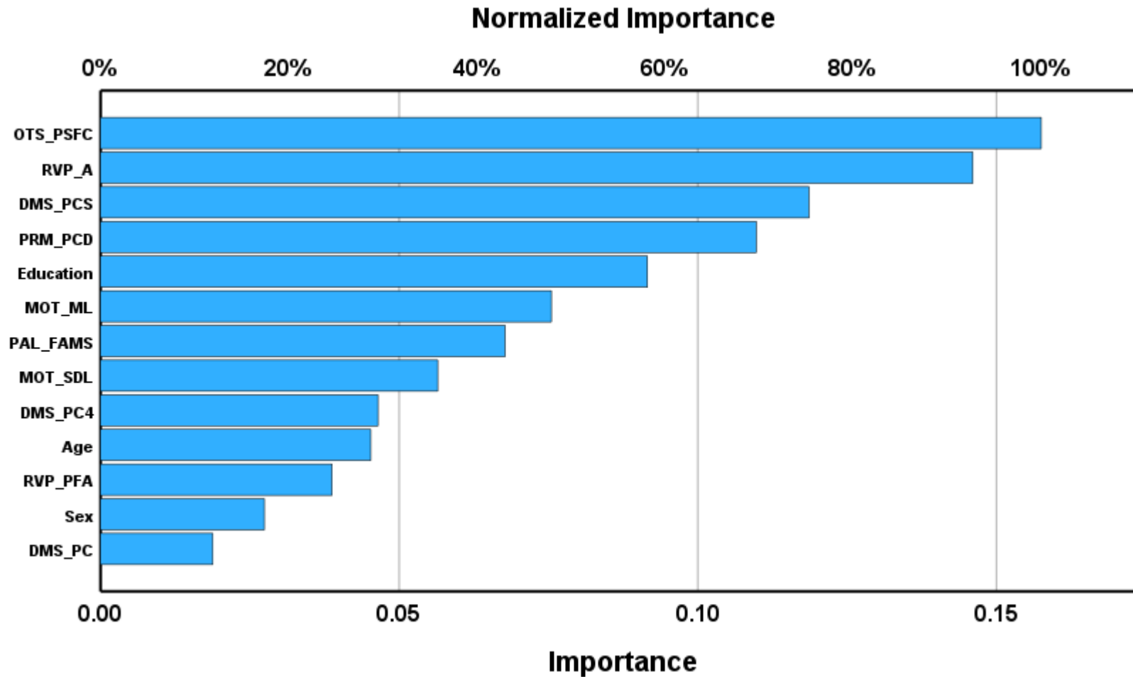
Figure 1. Results of neural network analysis with amnesic mild cognitive impairment and normal controls as output variables and selected key Cambridge Neuropsychological Test Automated Battery (CANTAB) test scores as input variables.
