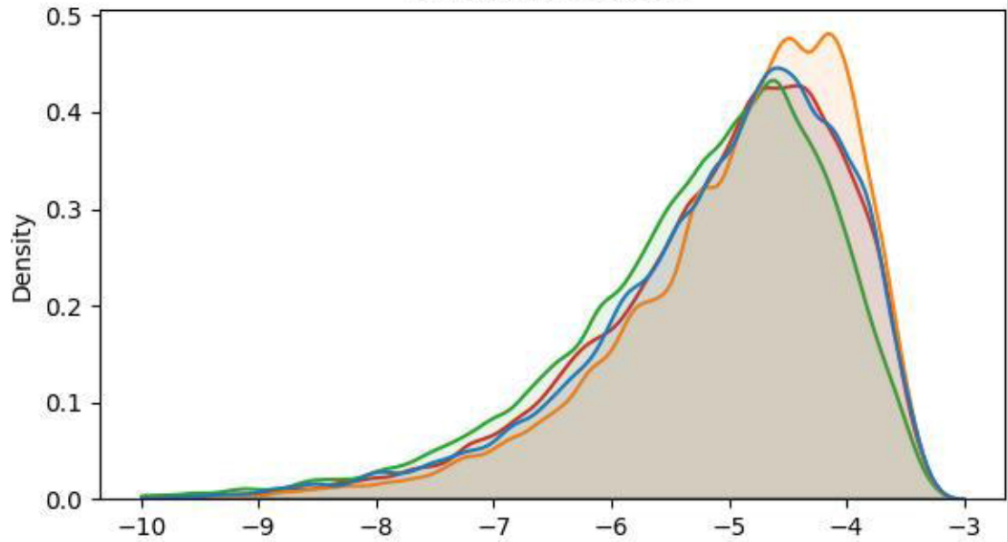
deaths contribution
