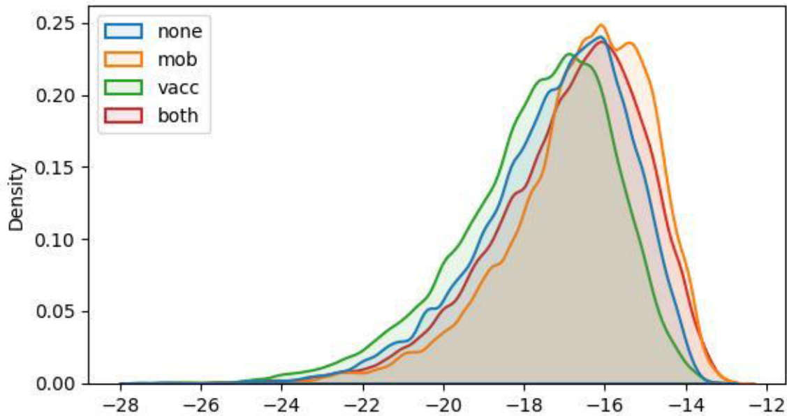
deaths contribution
