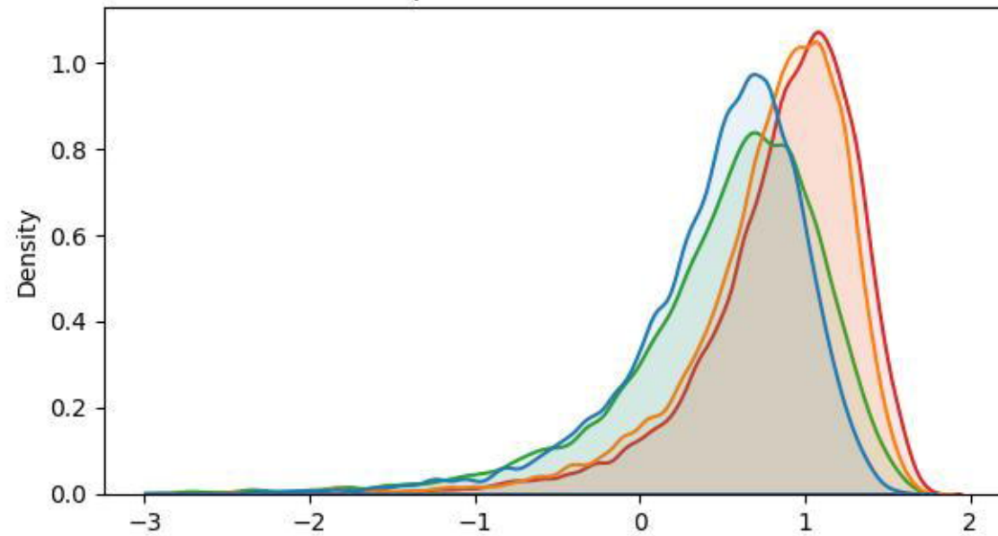
cases contribution
