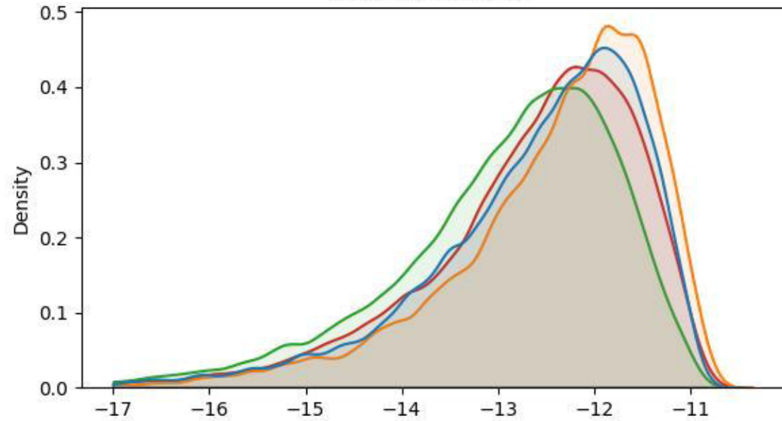
cases contribution
