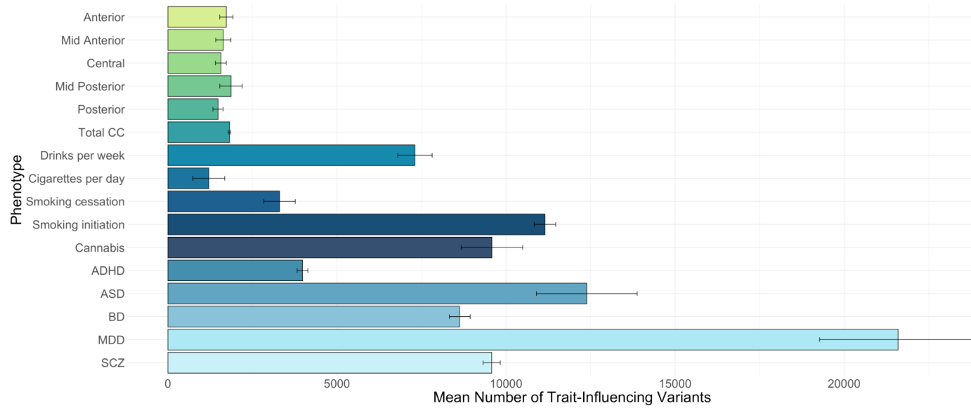
Figure 1: Polygenicity of the CC and psychiatric phenotypes illustrated by estimated causal variants
