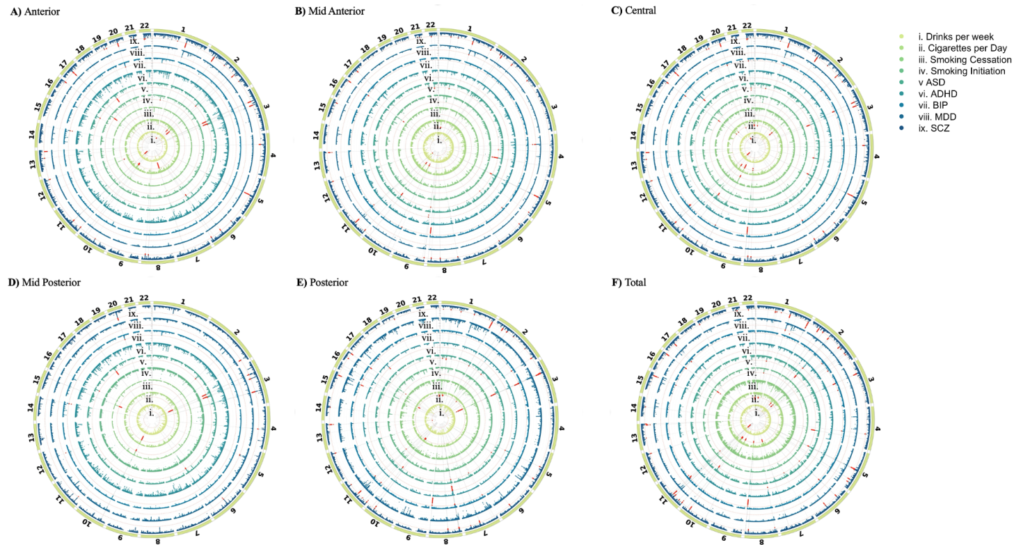
Figure 3: Manhattan plots of conjFDR results illustrated by subregion
