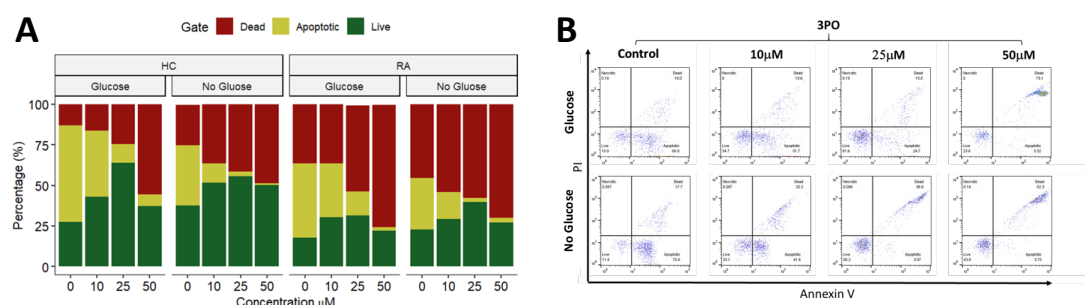
Figure 5. Effect of PFKFB3 inhibition with 3PO on neutrophil apoptosis. (A) Percentage of late apoptosis (red), early apoptosis (yellow) or live (green) HC and RA neutrophils incubated in glucose or no glucose media and treated for 24 h with varying concentrations of 3PO (0 – 50 \mu\text{M} ). (B) Representative flow cytometry traces for HC neutrophils showing annexin V and PI positive/negative gating.
