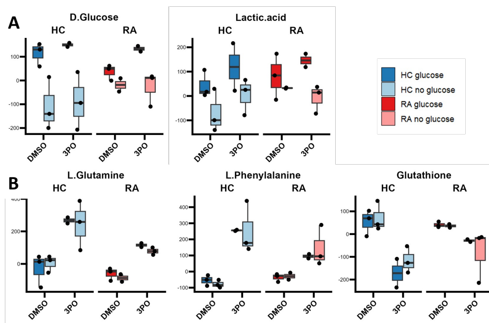
Figure 6. ^1\text{H} NMR analysis of RA and HC neutrophils with PFKFB3 inhibition by 3PO. Boxplots of metabolites measured by ^1\text{H} -NMR from neutrophils incubated in glucose or no glucose media for 4h with and without treatment with 50 \mu\text{M} 3PO. (A) The intracellular levels of glucose and lactic acid and (B) glutamine, phenylalanine and glutathione were affected by both glucose depletion and PFKFB3 inhibition by 3PO.
