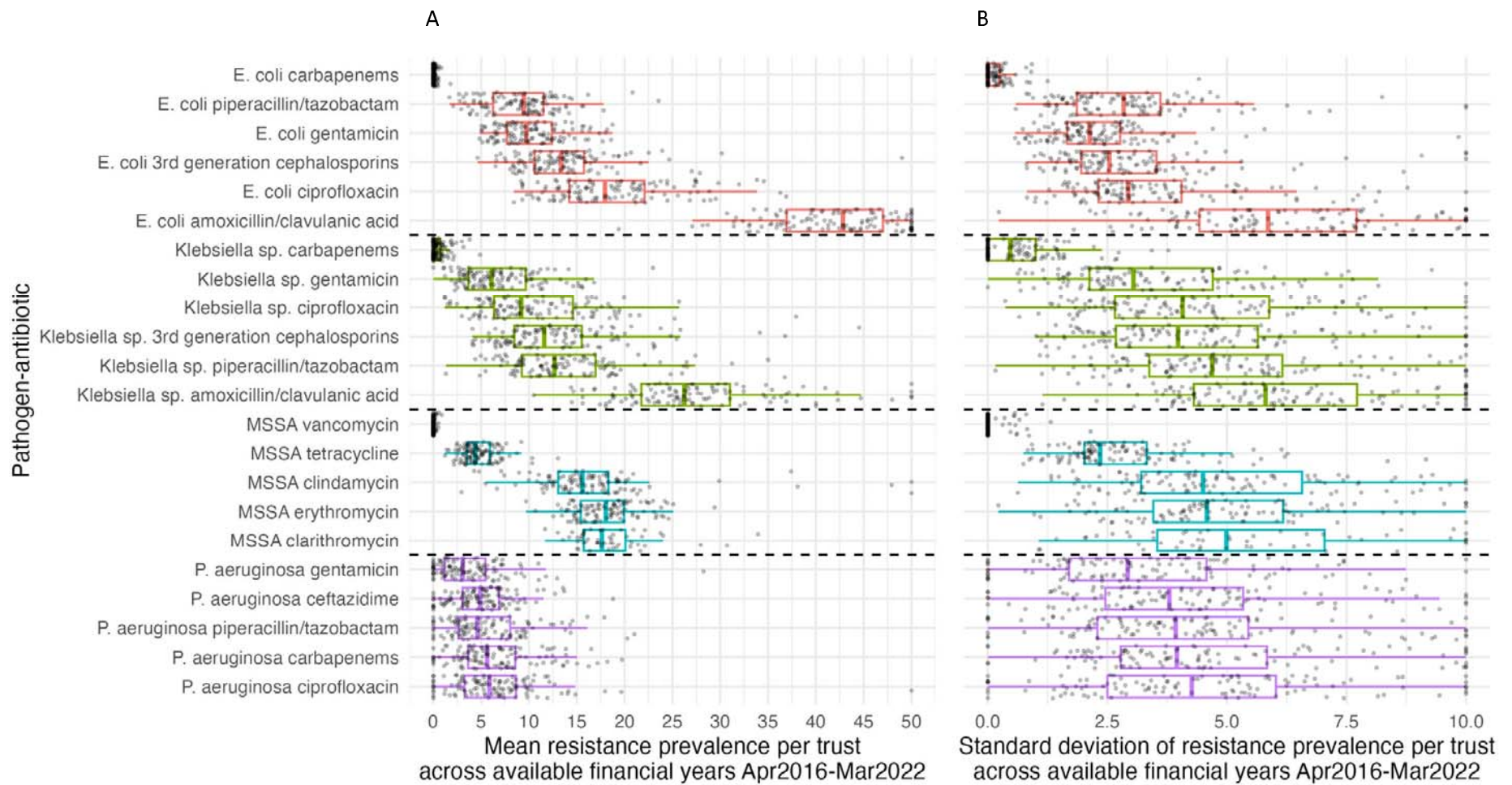
Figure 1 Distribution of mean resistance prevalence (A) and standard deviation (B) per Trust-pathogen-antibiotic across available financial years (Apr2016-Mar2022 for E. coli and MSSA and Apr2017-Mar2022 for Klebsiella sp. and P. aeruginosa ).
