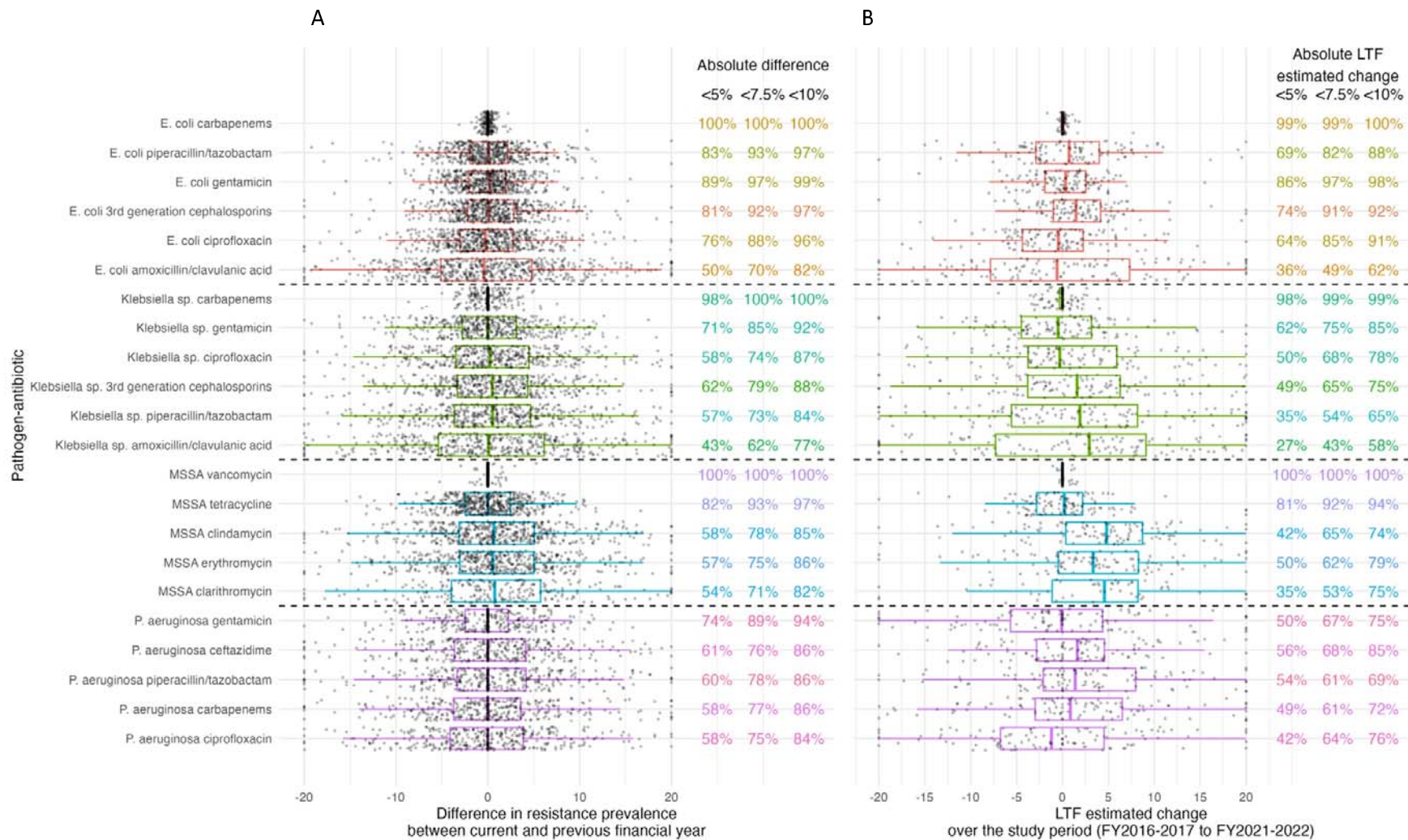
Figure 2 Distribution of difference in resistance prevalence between the current and previous financial year (A) and linear trend forecasting (LTF) estimated change over the study period (B), per pathogen-antibiotic combination across all Trusts and financial years. Percentages of Trust-FYs that have an absolute difference <5%, <7.5% and <10% between the current and the previous financial year are also given by pathogen-antibiotic combination (A), and an absolute LTF estimated change <5%, <7.5% and <10% (B).
