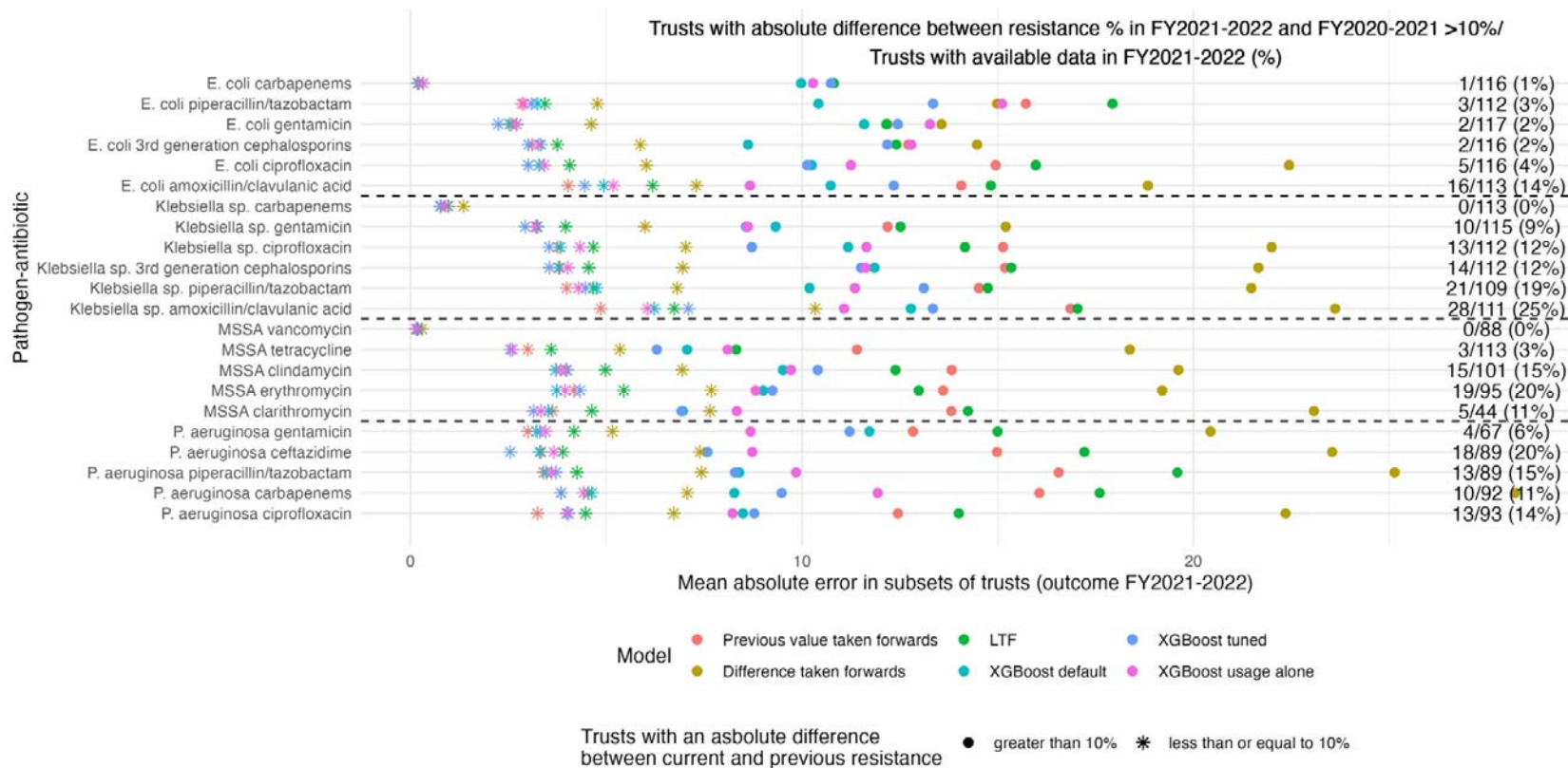
Figure 4 Mean absolute error for prediction on test set (resistance prevalence in FY2021-2022) for 6 different prediction models split by absolute difference between FY2021-2022 and FY2020-2021 in resistance prevalence, >10% or ≤10%
