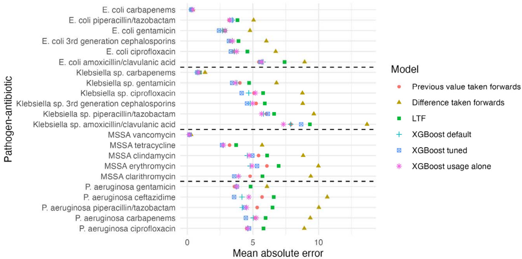
Figure 3 Mean absolute error for prediction on test set (resistance prevalence in FY2021-2022) for 6 different prediction models: taking the previous value forwards, taking the difference forwards, LTF, XGboost with default parameters, XGboost with tuned hyperparameters, XGboost with previous antibiotic usage alone as input features (no information on previous resistance prevalence).
