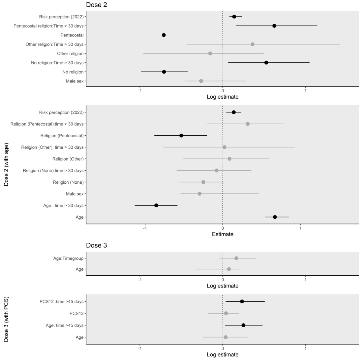
Figure S3: comparison between 2nd dose model with and without age, and 3 rd model with and without PCS12 score.
