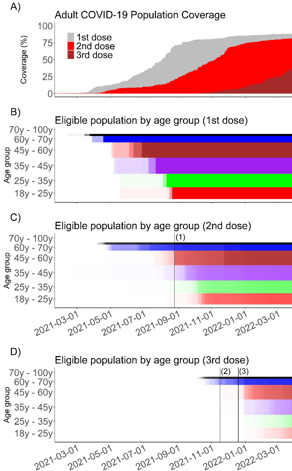
Figure 3: Summary of vaccination rollout in the community.
