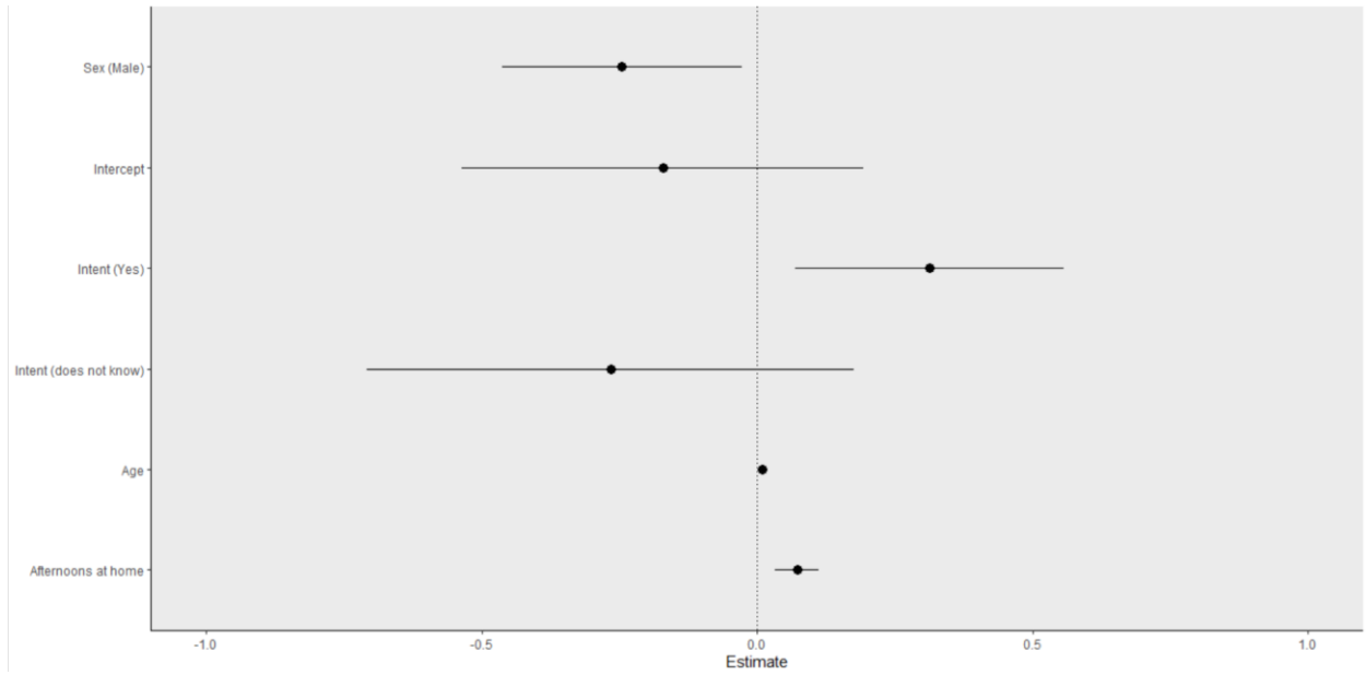
Figure S2: IPTW model results before resampling
