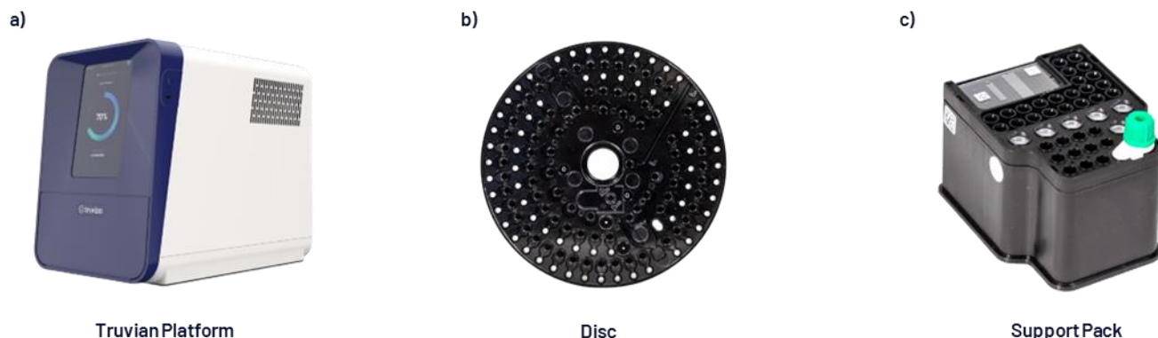
Figure 1. (a) Truvian Platform: an automated multi-modal blood testing analyzer measuring H = 17.25", L = 20", W = 12.5", (b) single-use disc consumable that contains microwells pre-filled with dried chemistries, plasma separation features, and hematocrit channel, (c) single-use support pack that holds the blood sample and contains pipette tips, buffers, reagent preparation wells, and a monolayer.
