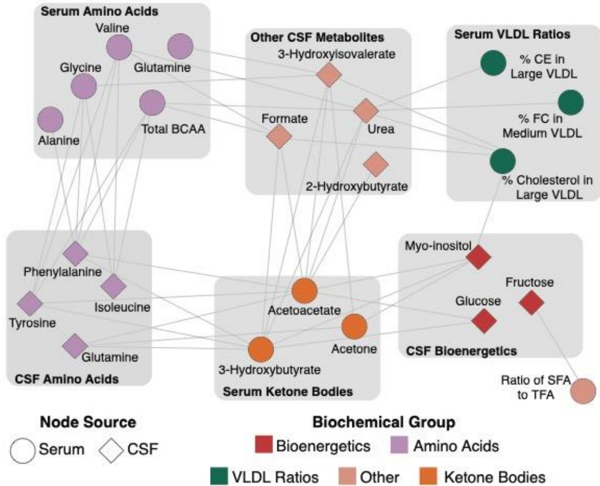
Figure 4: Bipartite graph between CSF and serum metabolites. Each node represents a metabolite. Ellipses depict metabolites measured in serum, and diamonds represent metabolites measured in CSF. Each edge represents a significant (FDR < 5%) correlation of the magnitude of changes pre- to post-diet between two metabolites. Node color represents their biochemical groups.
