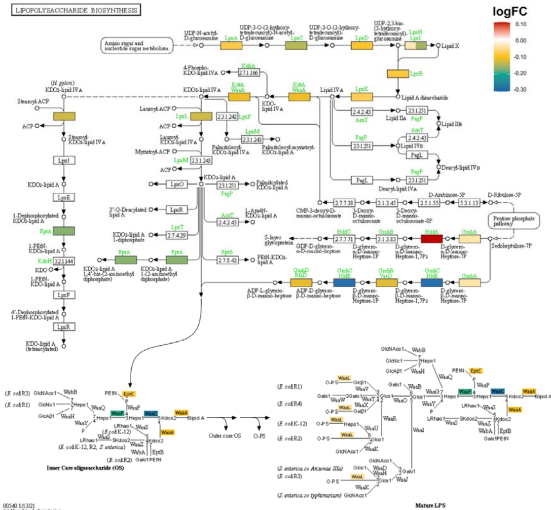
Figure 5: The lipopolysaccharide biosynthesis KEGG pathway (map00540 63 ) in maternal samples during the third trimester of pregnancy. Genes colored in yellow, green, and blue are incrementally less abundantly observed in the BEP-supplemented group. Genes colored in red are more abundantly observed in the BEP-supplemented group.
