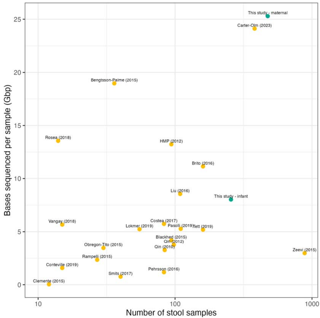
Figure S1: The number of samples versus the number of bases sequenced per sample for various gut metagenomic datasets and this study (adapted from (Carter et al., 2023) 64 ).
