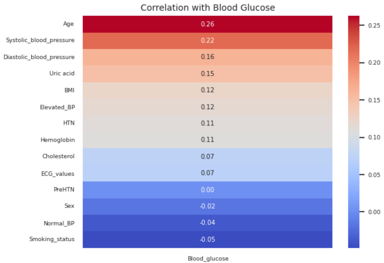
Figure 8: Correlation matrix of independent variables with the outcome variable
