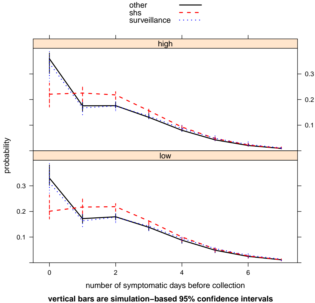
Figure 2: The model-estimated proportion of subjects with any given number of symptomatic days (from 0 to 7) prior to specimen collection, at each of two levels of community incidence, for each of three laboratory streams. The probability of symptom duration beyond 7 days was very low and is not shown. “shs” = student health service.
