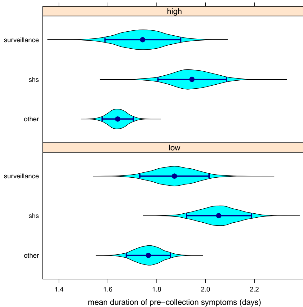
Figure 3: 5000 values of mean duration of symptoms simulated from the model, at each of two levels of community incidence, for each of three laboratory streams. Envelopes represent the density of the mean duration values obtained, while the dark bars show the means and their 95% two-sided confidence intervals. “shs” = student health service.
