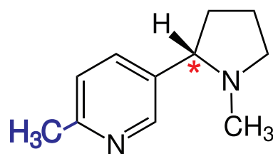
(S)-6-methyl nicotine
