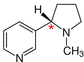
(S)-nicotine
