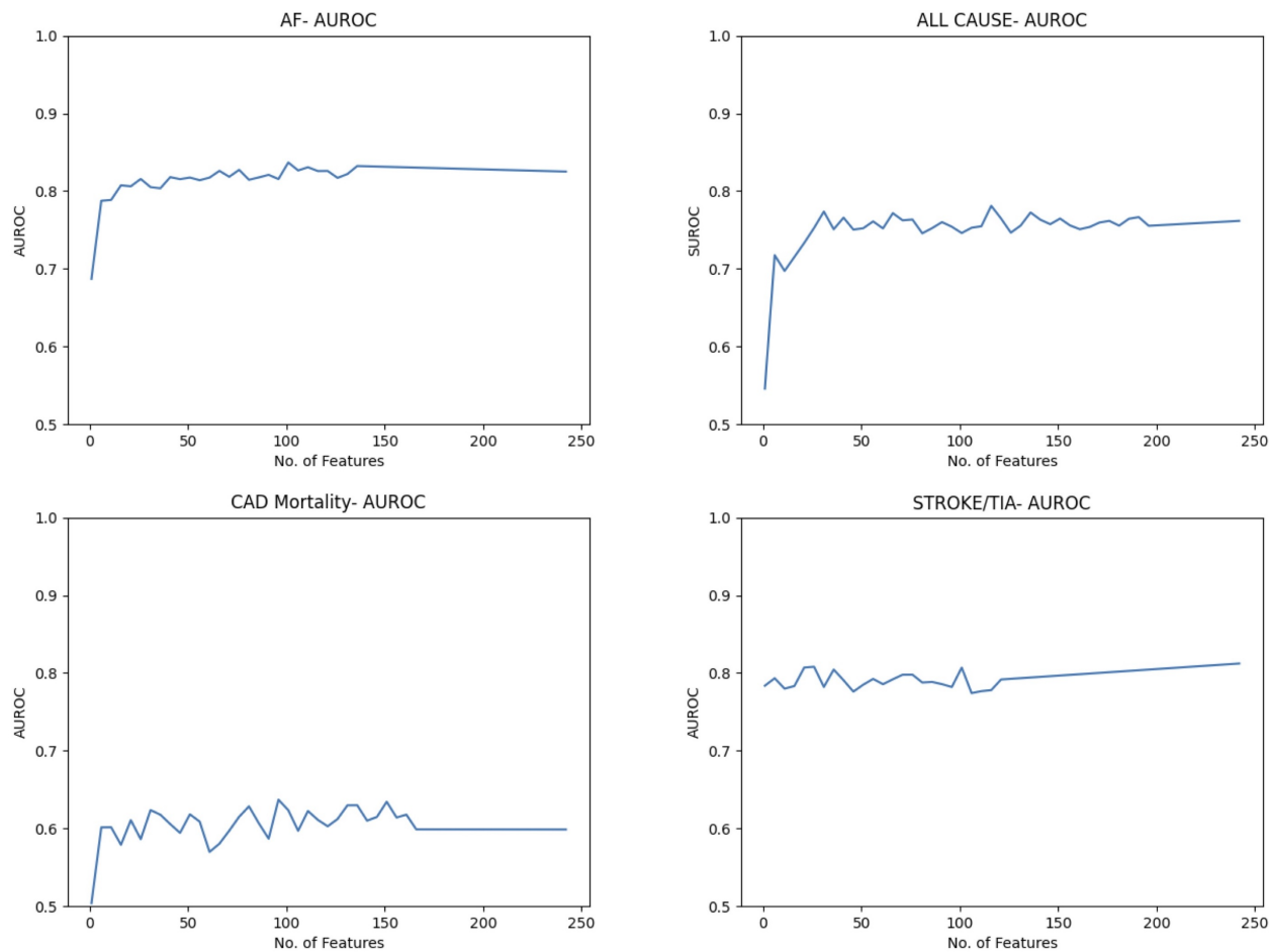
Fig. 5: Model performance (AUROC) for each outcome with addition of more features. AUROC values plotted of every 5 features added.
