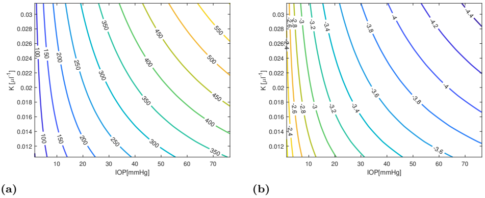
(a) (b) Fig 8. Frequency (a) and damping rate (b) of the slowest decaying mode as a function of IOP and ocular rigidity K .
