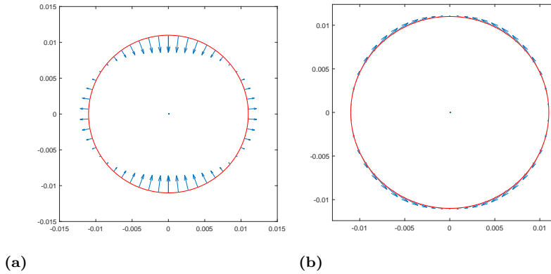
Fig 2. Velocity fields on the boundary corresponding to the two eigenvalues from (28) for \ell = 2 and m = 0 .
