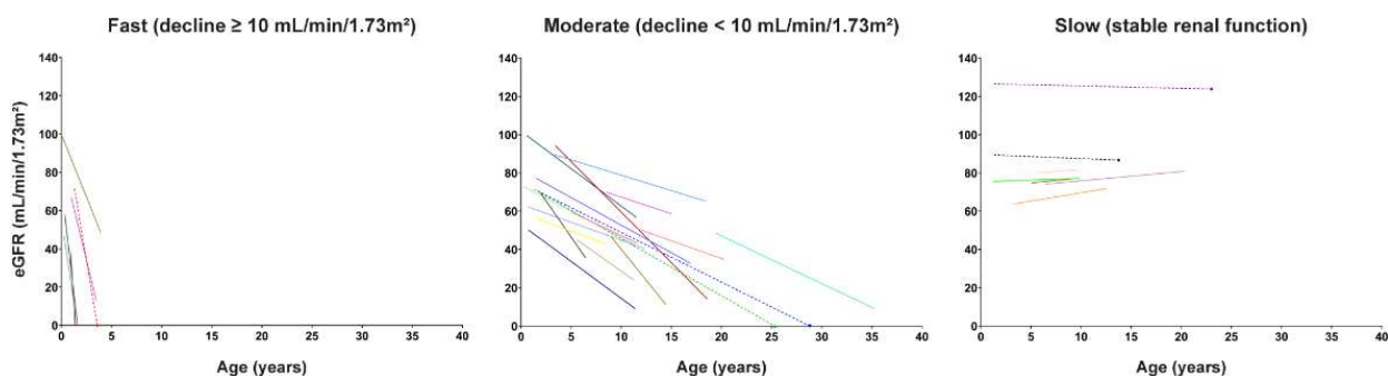
Figure 1. Annual renal function decline. Patterns of eGFR change over time were plotted for each patient and stratified as fast, moderate or slow according to the curve slopes determined by linear regression. Each coloured line indicates the annual eGFR loss. Dashed lines indicate patients for whom we only had one value of eGFR corresponding to the last follow-up.
