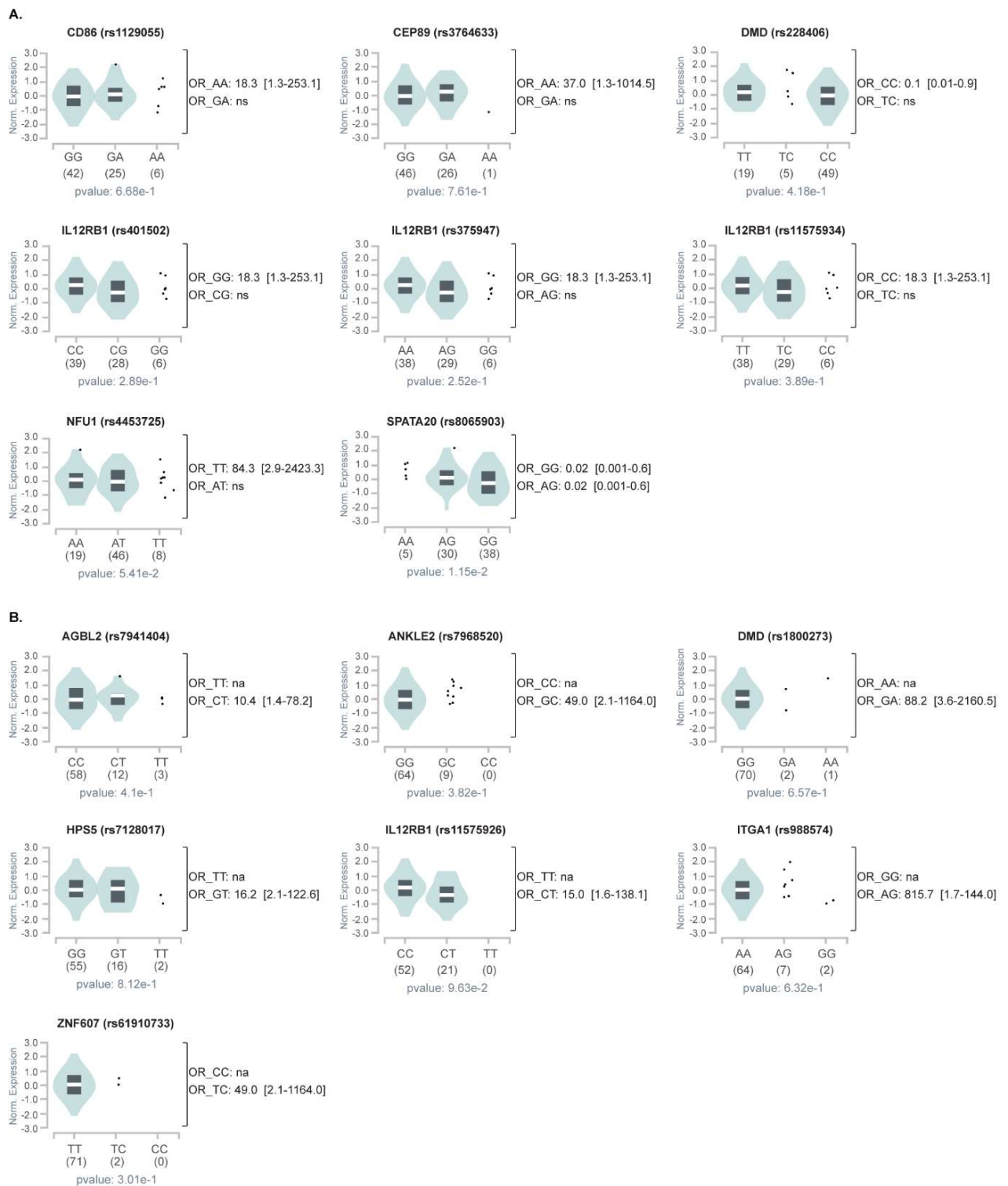
Figure 4. Violin plots of allele-specific cis-eQTLs according to genotypes for each significant variant in human kidney cortex tissues from the GTEx database. The teal region indicates the density distribution of the samples in each genotype. The allelic effect of variants on normalized gene expression levels are shown by boxplots within violin plots. The white line in the box plot (black) shows the median value of the expression of each genotype. The alleles and number of subjects analysed is shown under each genotype. A. Variants in homozygosity for the alternative allele associated to fast renal progression. B. Variants in heterozygosity associated to fast renal progression. The odds ratio and 95% confidence intervals calculated from table 2 are shown next to each plot for reference.
