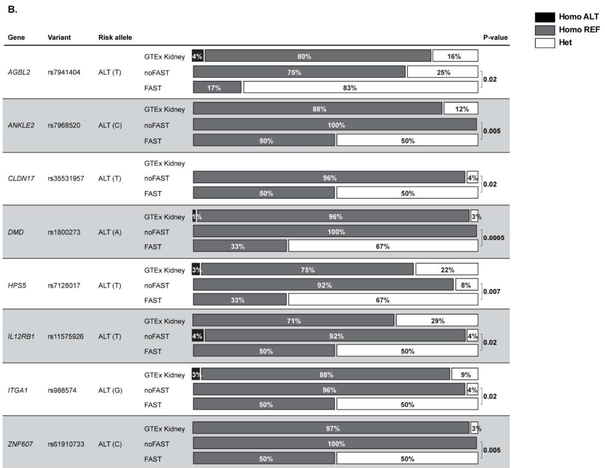
Figure 5. Distribution of the three possible genotypes for each candidate modifier gene variants across two FHHNC phenotypes and the control group from GTEx. A. Variants in homozygosis for the alternative allele associated to fast renal progression. B. Variants in heterozygosis associated to fast renal progression. Comparisons were performed by the Fisher's exact test.
