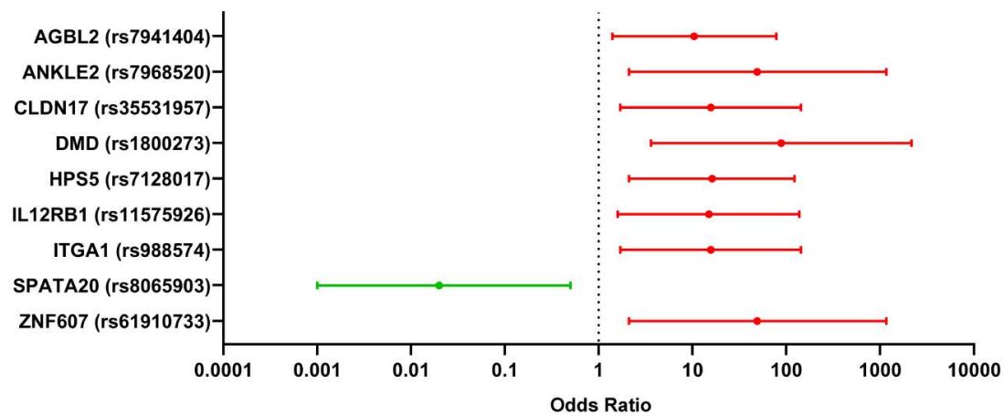
Figure 3. Forest plot showing the significant variants in candidate modifier genes associated to the FAST phenotype of FHHNC patients. A. Odds ratios and 95% confidence intervals were calculated by comparing the distribution of the alternative allele in homozygosis versus the reference allele in homozygosis. B. Odds ratios and 95% confidence intervals were calculated by comparing the distribution of the alternative allele in heterozygosis versus the reference allele in homozygosis.
