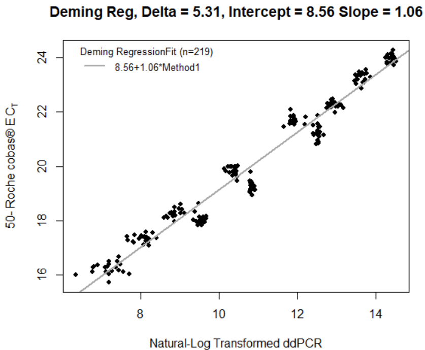
Figure 3. Deming Regression of Data without outliers with log-transformed ddPCR GE/ml on the x-axis and 50 – Roche cobas® E CT on the y-axis, using the computed average ratio of the variances as our delta.
