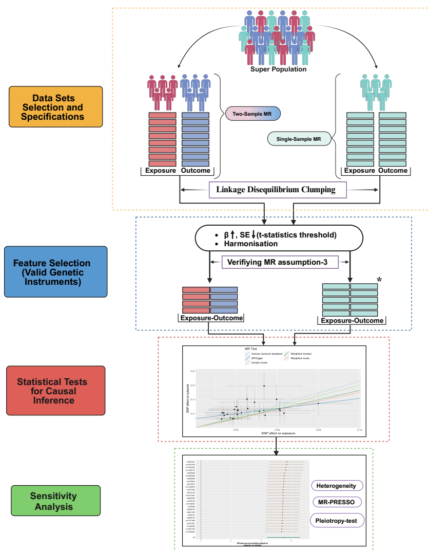
Figure 2: Proposed workflow
