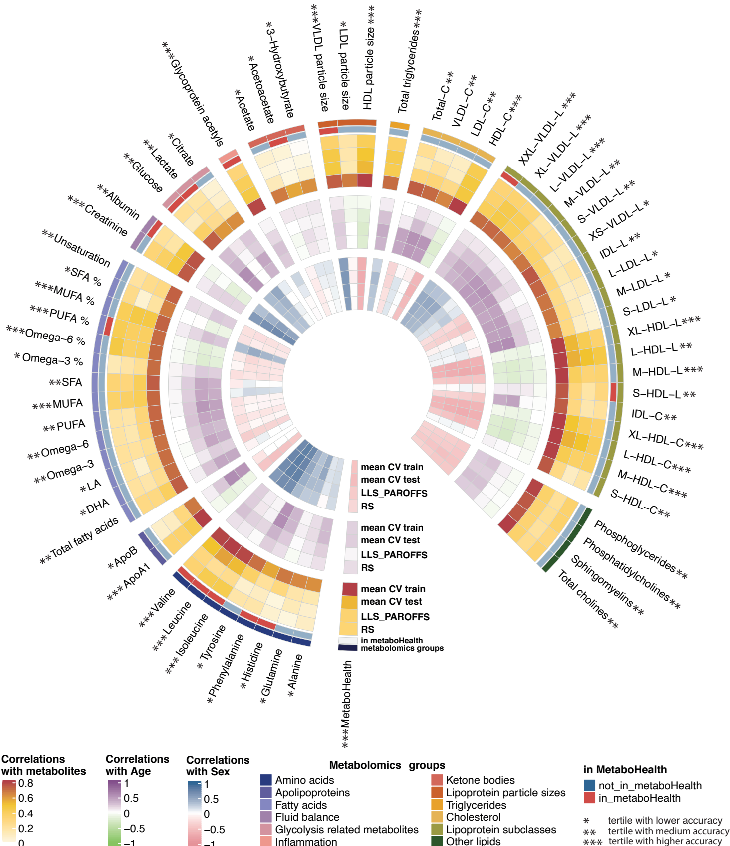
Figure 3: DNAm metabolomics accuracies
