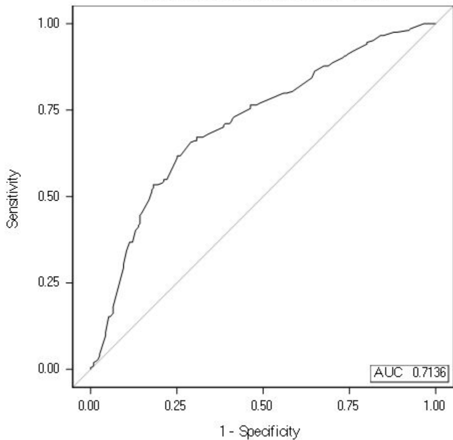
Multivariate Regression ROC Curve
