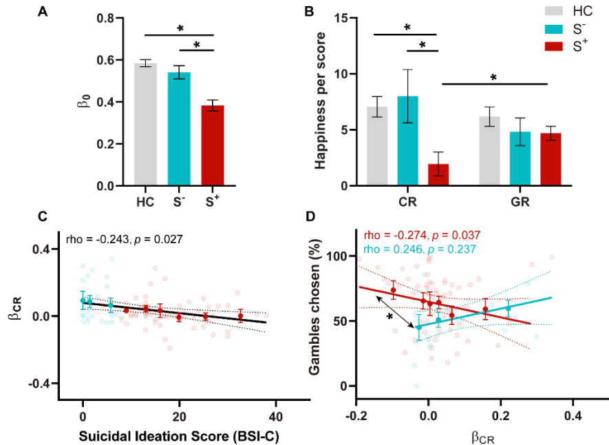
Figure 3. Effect of Suicidal thoughts and behavior on mood dynamics. A) Group difference in mood baseline, \beta_0 . B) Group differences in mood sensitivity to certain reward (CR) and gamble reward (GR). C) Correlation between Suicidal Ideation score at current time BSI-C and mood sensitivity to CR. D) Correlational difference in S^- and S^+ between mood sensitivity to CR and gambling behavior. Abbreviations: CR, certain reward; GR, gamble reward; HC, healthy control; S^- , patients without suicidal thoughts and behavior; S^+ , patients with suicidal thoughts and behavior; BSI-C, Beck Scale for Suicidal Ideation at the current time; *p < 0.05 .
