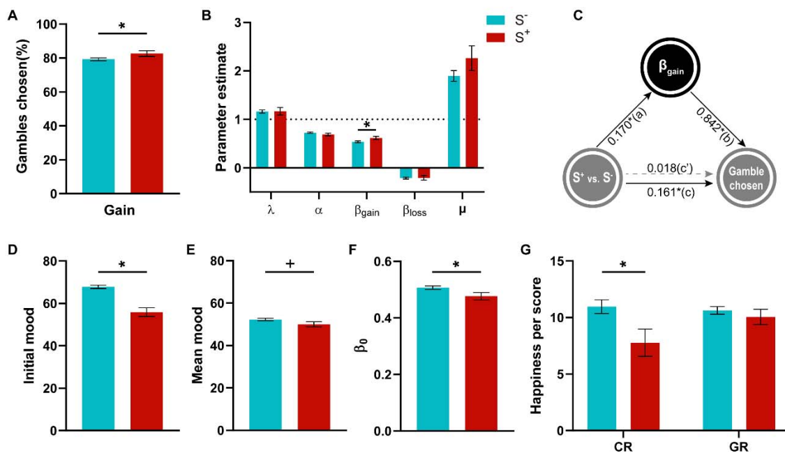
Figure 4. Validation of suicidal-related results in an independent dataset of healthy populations (n = 747).
