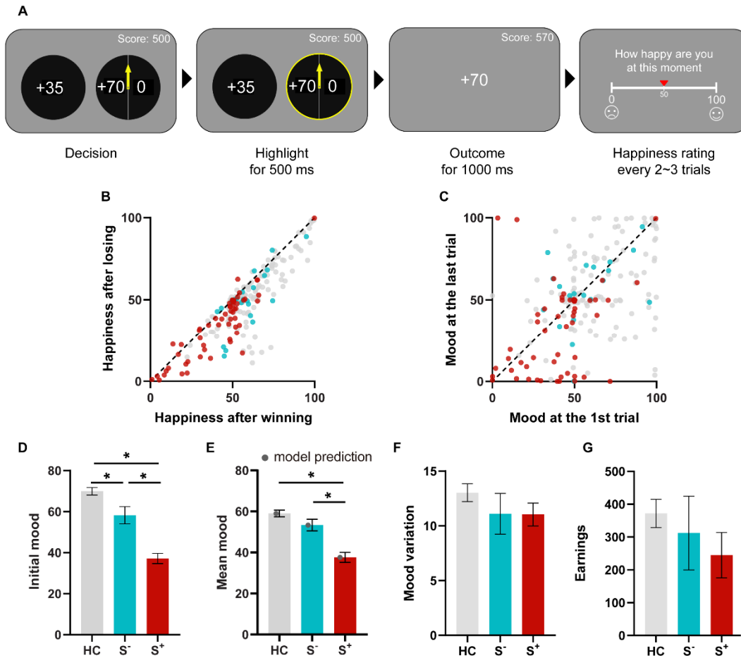
Figure 1. Task design, outcome and time effects on mood, and group differences in mood. A) Gambling task with mood ratings. On each trial, participants were asked to choose between a certain option and a gambling option (self-paced). Once selected, the chosen option was highlighted in yellow for 500 ms. Then the corresponding outcome was displayed in the center of the screen for 1000 ms. The cumulated score was always shown in the right-upper corner. Every 2 to 3 trials, participants were asked to complete a self-paced rating of their happiness, answering the question “How happy are you at the moment” on a slider from 0 (very unhappy) to 100 (very happy). B) Patients and healthy controls felt happier after winning than losing. C) Mood drifted over time. D) Group difference in mood before the task show weakened mood in S + . E) Group difference in average mood displays lower mood experience in S + . The grey dots represent the winning model predictions. F) Mood variance was similar for all the three groups, as indexed by standard deviation of happiness ratings across the task. G) Each group earned about the same amount of point by the end of the task. Abbreviations: HC, healthy control; S - , patients without suicidal thoughts and behavior; S + , patients with suicidal thoughts and behavior; * p < 0.05 . Error bars correspond to the standard error.
