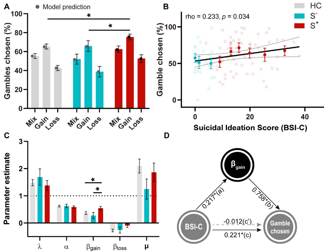
Figure 2. Choice results. A) Group differences in gambling behavior. The grey dots represent the winning model prediction. B) Positive correlation between Suicidal Ideation score at current time (BSI-C) and gambling behavior in patients. C) The estimated parameters from the winning choice model differed across groups, with higher approach behavior for S + . D) The mediation model among the BSI-C, \beta_{gain} , and gambling behavior in the gain condition among patients. The Pavlovian approach parameter mediated the effects of BSI-C on increased gambling behavior in the gain condition. Abbreviations: HC, healthy control; S - , patients without suicidal thoughts and behavior; S + , patients with suicidal thoughts and behavior; BSI-C, Beck Scale for Suicidal Ideation at the current time; * p < 0.05 .
