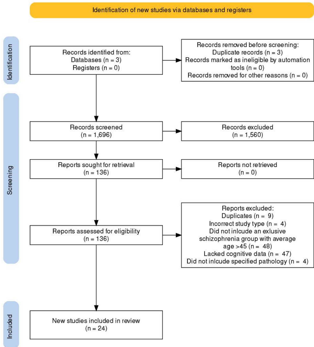
Figure 1: PRISMA flowchart
