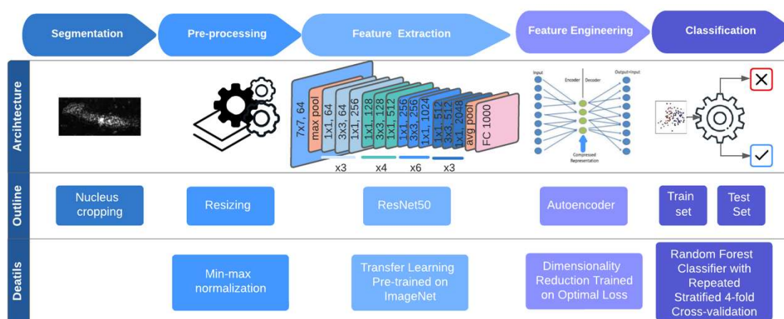
Figure 7. Workflow and architecture of the AI driven feature engineering model
