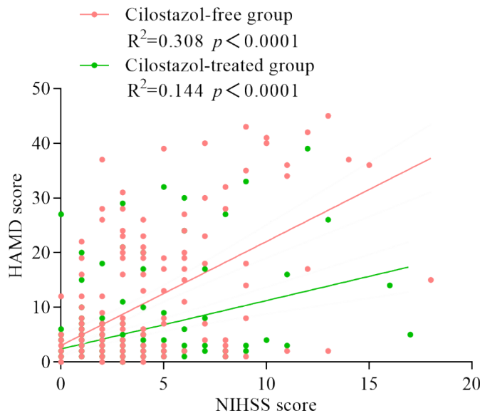
Figure 4. Correlation analysis between NIHSS score and HAMDS score in patients of the cilostazol-free group and cilostazol-treated group at the end of follow-up. Spearman rank correlation test was used to analyze the correlation between NIHSS score and HAMDS score. R^2 is the determining coefficient. The higher R^2 is, the stronger the correlation between NIHSS score and HAMDS score is. p < 0.0001 indicates that the correlation coefficient R has extremely significant statistical significance.
