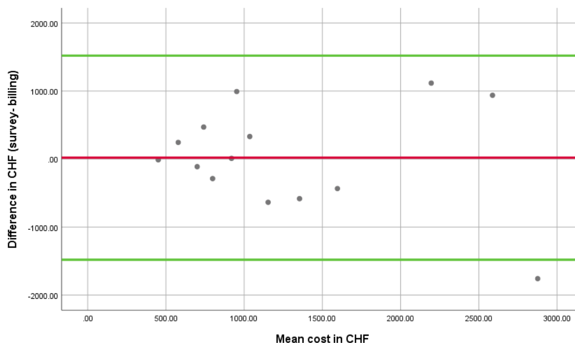
Figure 1 Bland Altman Plot
