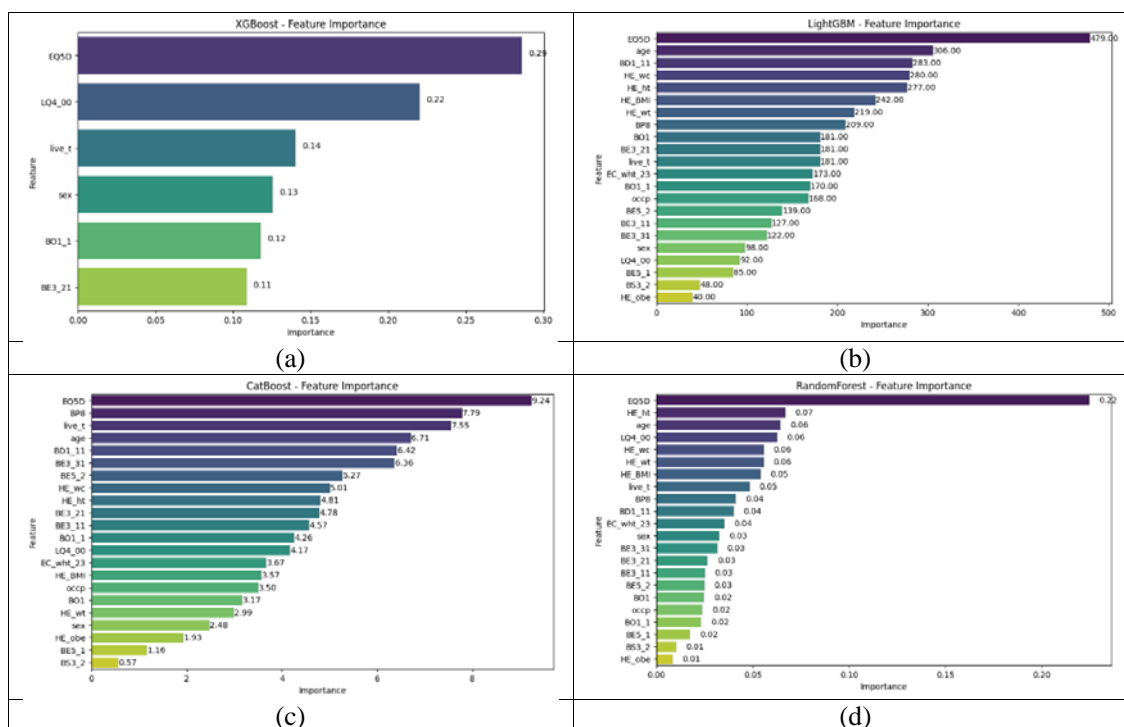
Figure 3. Feature importance: XGBoost (a), LGBM (b), CatBoost (c), RandomForest (d)
