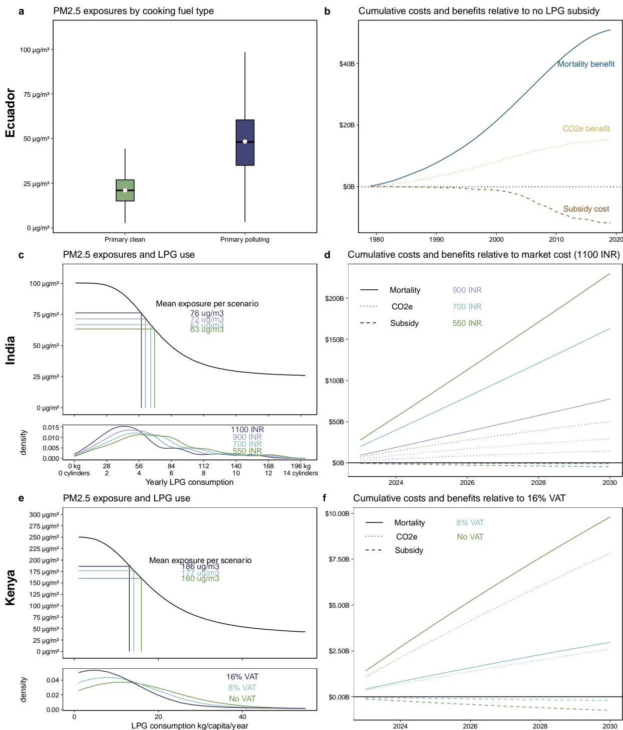
Figure 1. Benefits from LPG subsidies outweigh associated costs across three case studies in Ecuador, India, and Kenya. Panels a and b describe the data and results for Ecuador. Panel a shows the distribution of 1,000 average annual PM2.5 exposure estimates for those living in households that rely on clean burning fuels (namely gas) as compared to those that rely on biomass primarily. Panel b indicates calculated cumulative mortality benefits, CO2e-related benefits, and costs related to subsidizing gas in USD relative to the counterfactual scenario where there was no LPG subsidy. Panels c and d describe the data and results for India. Panel c
