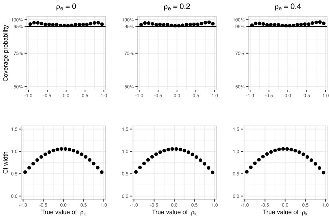
Figure 3: Setting environmental correlation between error terms has no effect on genetic correlation estimates.
