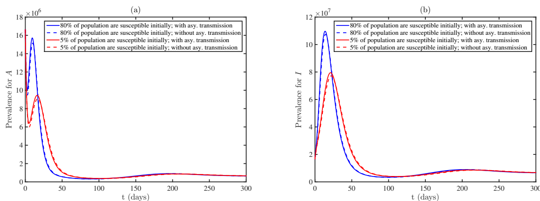
Figure 2. Convergence to the endemic equilibrium for model (2.1) with \mathcal{R}_c = 5.352 . The parameter values are detailed in Table 1. The solid lines depict the disease dynamics with varying proportions of susceptible individuals at the outset. The dashed lines represent the scenario without asymptomatic transmission.
