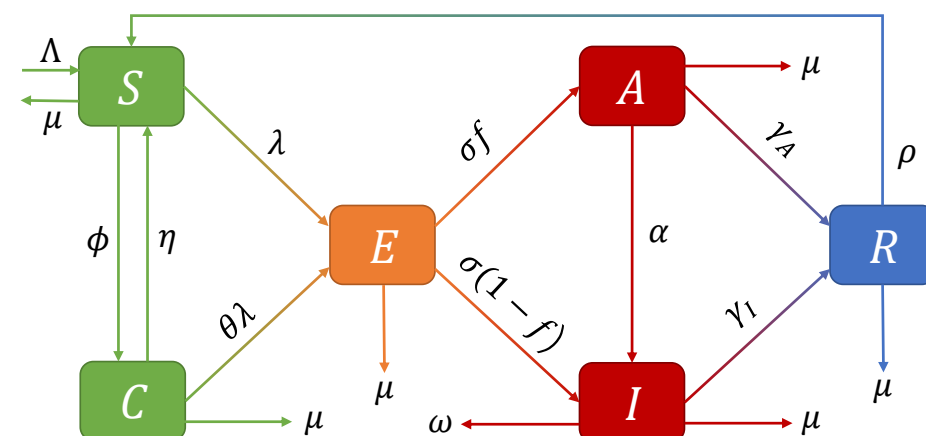
Figure 1. Flow diagram of model (2.1). The population is divided into 6 compartments: susceptible individuals (S), vaccinated individuals (C), exposed individuals (E), asymptomatic infected individuals (A), symptomatic infected individuals (I), and recovered individuals (R). Detailed model parameter descriptions are given in Table 1.
