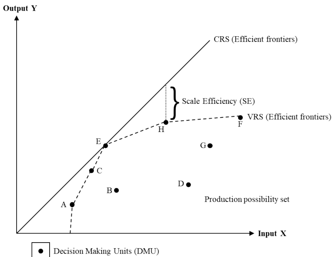
281 Fig 2. Concepts of efficiency measurement in Data Envelopment Analysis
