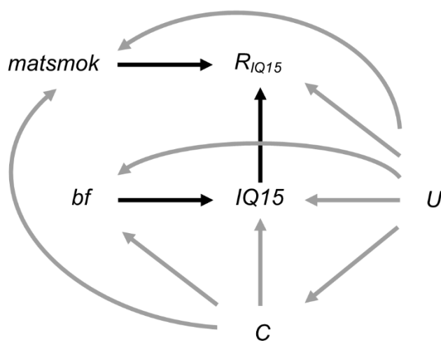
Figure 8. Directed acyclic graph depicting the relationship between child’s IQ at age 15 years ( IQ15 ), duration of breastfeeding ( bf ), confounders of the IQ15 - bf relationship ( C ), whether the mother smoked during the first trimester of pregnancy ( matsmok ), missingness indicator R_{IQ15} (a binary variable indicating whether IQ15 is observed), and unmeasured variable(s) U . Lines indicate related variables, with arrows indicating the direction of the relationship. Black lines depict the relationships assumed in theoretical Scenario 1; grey lines depict additional relationships that are plausible in our real data example; absent lines represent variables with no direct causal relationship.
