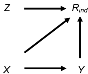
Figure 5. Directed acyclic graph depicting the relationship between outcome Y , exposure X , missingness indicator R_{ind} , and potential auxiliary variable Z . Lines indicate related variables, with arrows indicating the direction of the relationship; absent lines represent variables with no direct causal relation
