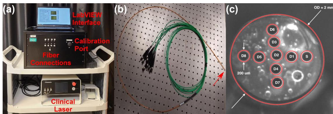
Figure 1: (a) Image of spectroscopy system showing fiber connections for source and detector fibers, port for integrating sphere calibration, LabVIEW interface, and the laser used for clinical PDT. (b) Image of fiber optic probe, with distal tip indicated by red arrow. (c) Image of fiber optic probe distal face showing the 200 \mu\text{m} diameter fibers used for delivery and detection of light. The source fiber is labeled “S,” detector fibers are labeled “D,” and outside diameter is abbreviated as “OD.”
