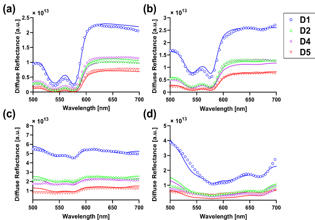
Figure 2: Corrected diffuse reflectance data (open circles) and fits (solid line) for detector fibers 1, 2, 4, and 5 for Subject 3 (a) pre-MB and (b) post-MB, and Subject 8 (c) pre-MB and (d) post-MB. Colors and symbols indicate different detector fibers.
