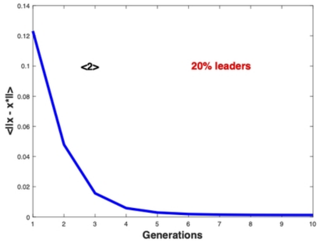
Covergence to equilibrium \langle \|x - x^*\| \rangle \leq 0.00125
