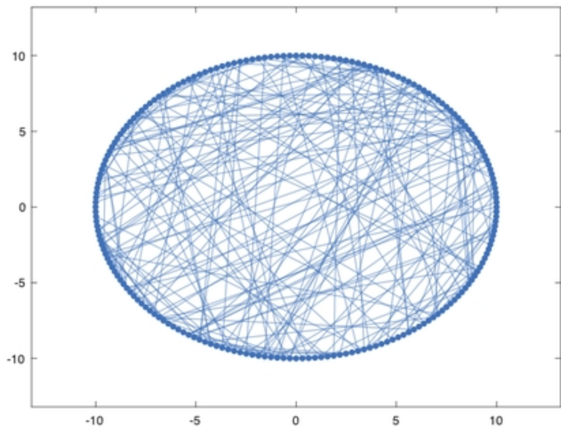
Small World Network: m = 200 , K = 6 , b = 0.3
