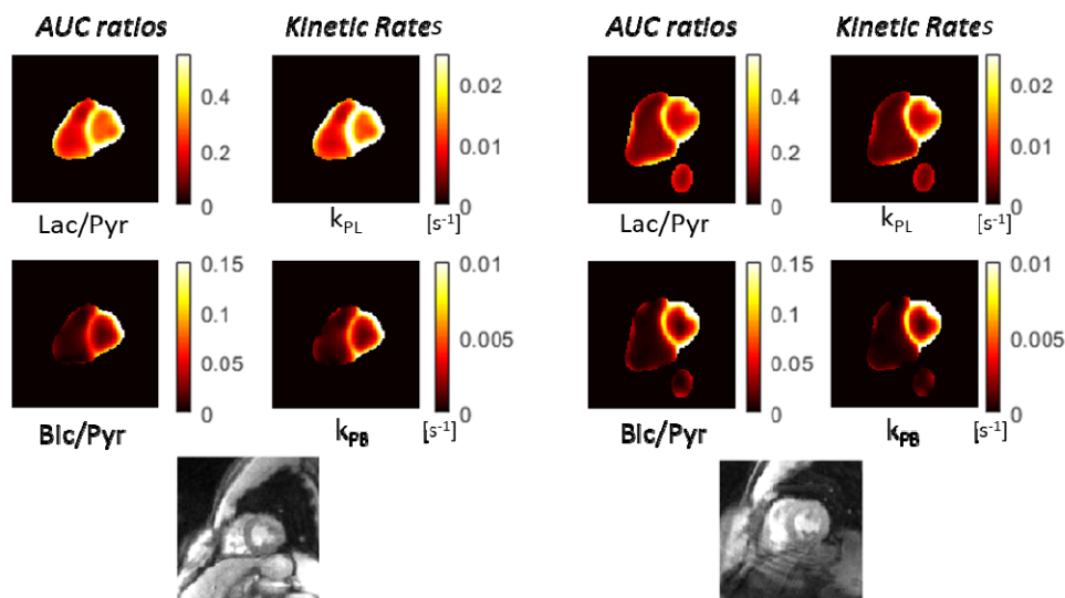
Figure 4: Quantification using AUC ratios and pharmacokinetic modeling in the same healthy volunteer subjects as Fig. 3 (subjects HV6, left, and HV7, right). k_{PL} is the 13 C-pyruvate to 13 C-lactate rate and k_{PB} is the 13 C-pyruvate to 13 C-bicarbonate rate. Note the maps are only computed in regions that meet a minimum pyruvate AUC SNR threshold as pyruvate signal is required for these quantifications.
