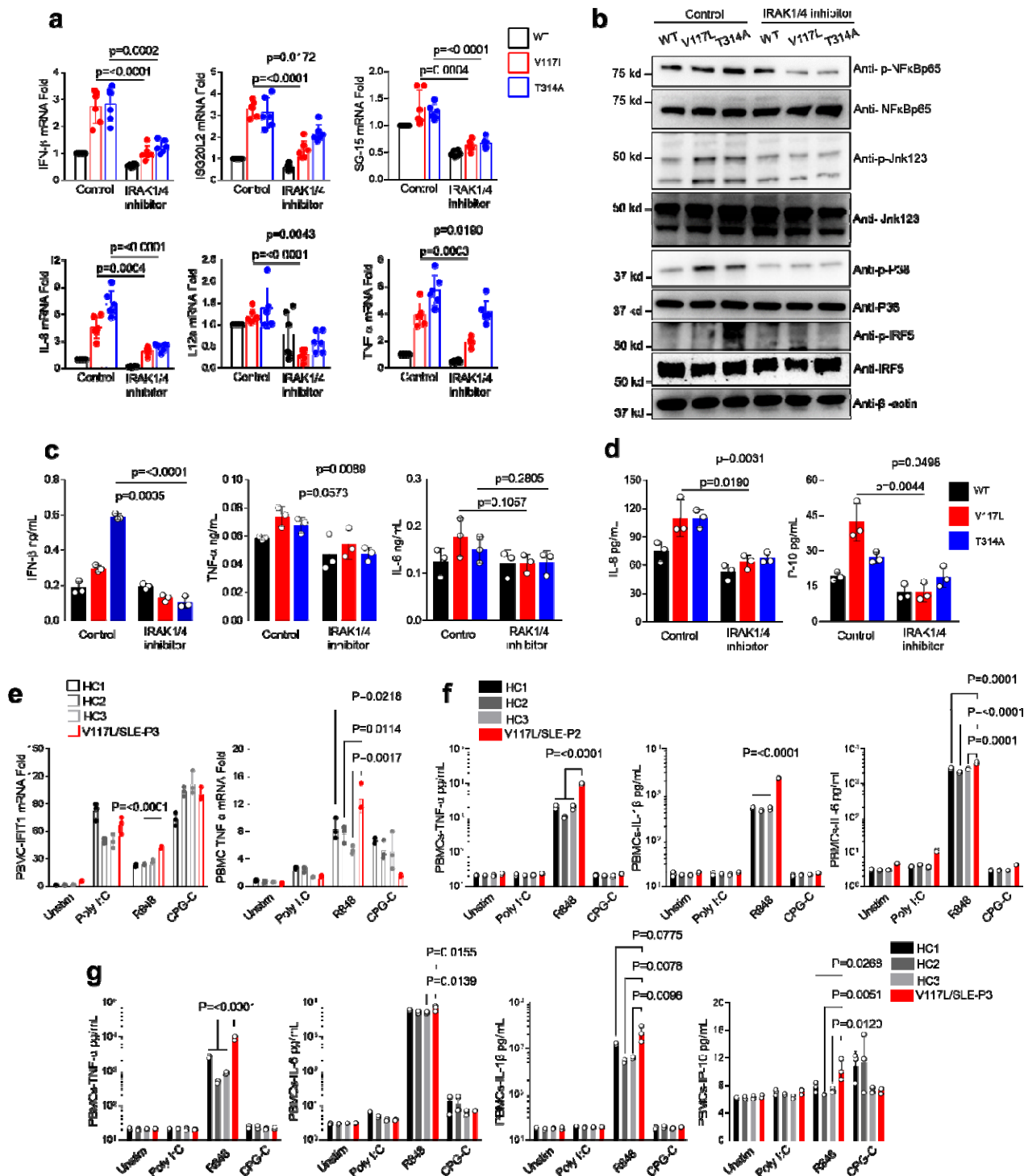
Fig. 4 UNC93B1 genetic variation drive inflammation via TLR7/IRAK1/4 axis. (a) Quantitative RT-PCR analysis of IFN \beta , ISG20L2, ISG-15, IL-8, IL-12a, and TNF \alpha expression in the indicated THP-1 cell lines after incubation with IRAK1/4 inhibitor for 24hrs, n=3 biological replicates. Data are representative of two independent experiments. (b) Levels of phosphorylated NF \kappa B, JNK1,2,3, p38, and irf5 as measured by immunoblot using lysates of the indicated THP-1 cells after incubation with IRAK1/4 inhibitor for 24hrs. (c) Production of IFN \beta and TNF \alpha in the indicated THP-1 cell lines after incubation with IRAK1/4 inhibitor for 72hrs. n=3 biological replicates. (d) Production of IL-8 and IP-10 in the indicated THP-1 cell lines after incubation with IRAK1/4 inhibitor for 72hrs. n=3 biological replicates (CBA).
